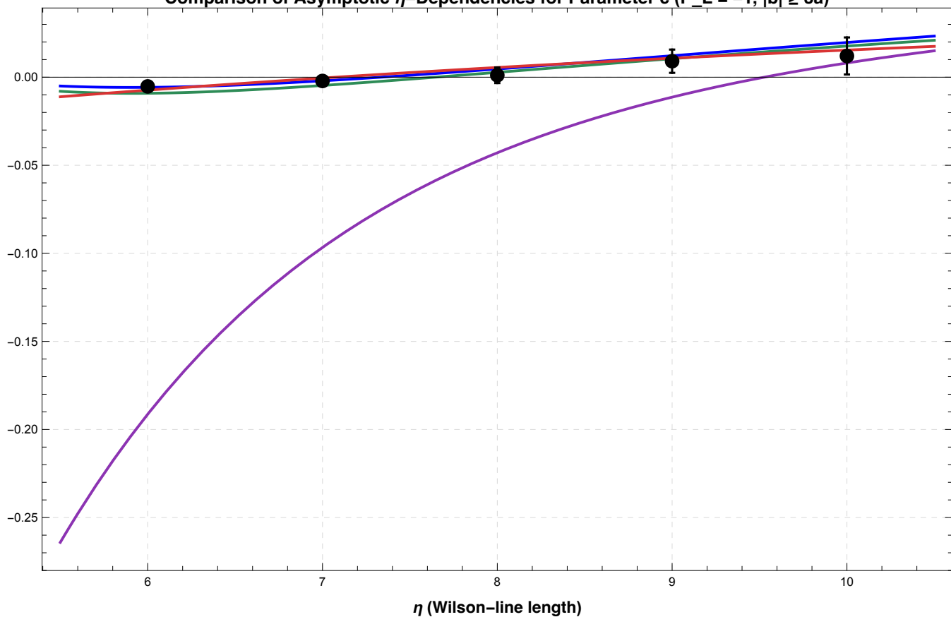
Comparison of Asymptotic \eta -Dependencies for Parameter c ( P_L = -1, |b| \geq 3a )
