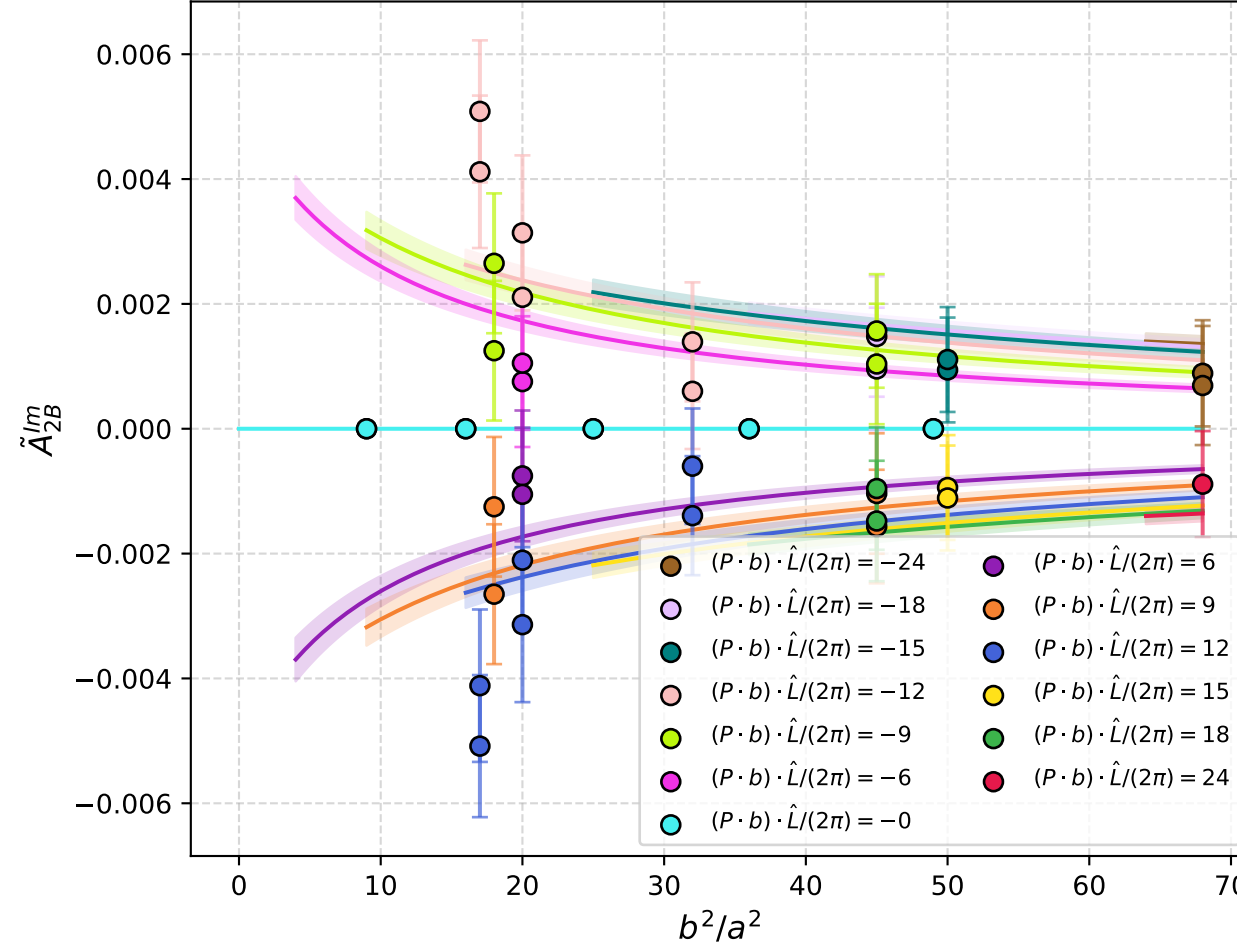
\tilde{A}_{2B}^{\text{Im}} vs b^2/a^2
