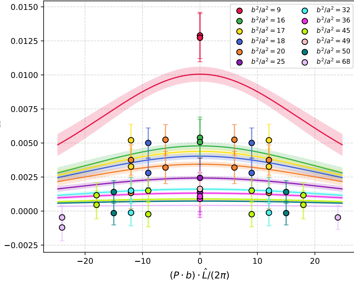
\tilde{A}_{2B}^{\text{Re}} vs b^2/a^2
