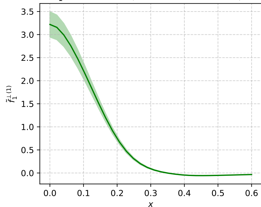
\tilde{f}_1^{\perp(1)} = -2\tilde{A}_{12B} (\hat{\zeta} \rightarrow \infty, b^2=9.0) [c + d/\hat{\zeta}]
