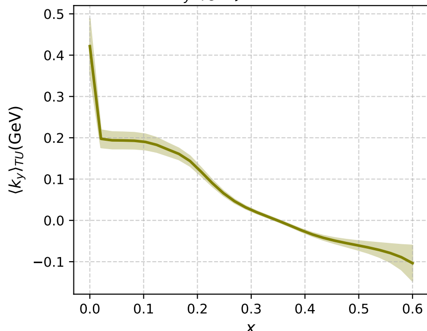
Sivers Shift \langle k_y \rangle_{TU} (\hat{\zeta} \rightarrow \infty, b^2=9.0) [c + d/\hat{\zeta}]
