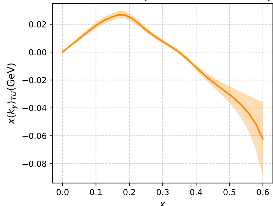
x^* \text{ Sivers Shift } (\hat{\zeta} \rightarrow \infty, b^2=9.0) [c + d/\hat{\zeta}]
