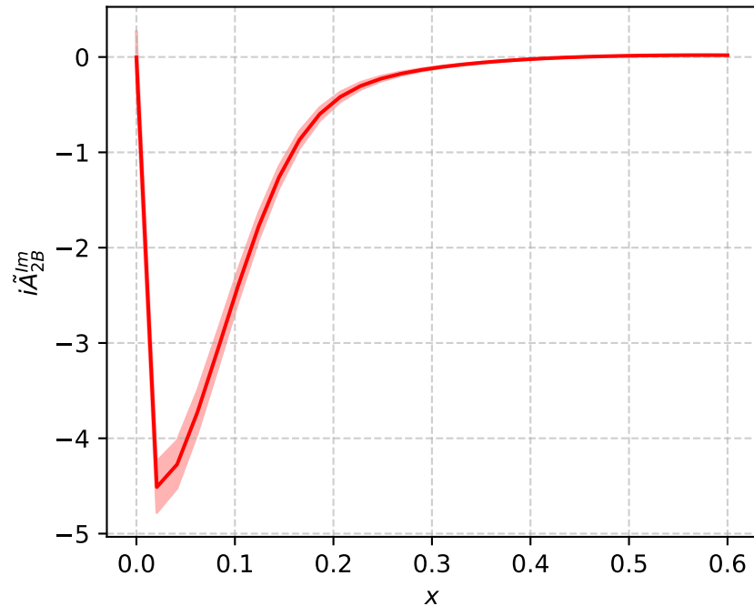
i\tilde{A}_{2B}^{Im} (\hat{\zeta} \rightarrow \infty, b^2=9.0) [c + d/\hat{\zeta}]
