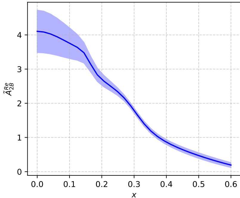
\tilde{A}_{2B}^{Re} (\hat{\zeta} \rightarrow \infty, b^2=9.0) [c + d/\hat{\zeta}]
