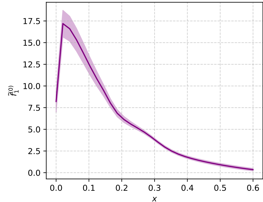
\tilde{f}_1^{(0)} = 2\tilde{A}_{2B} (\hat{\zeta} \rightarrow \infty, b^2=9.0) [c + d/\hat{\zeta}]
