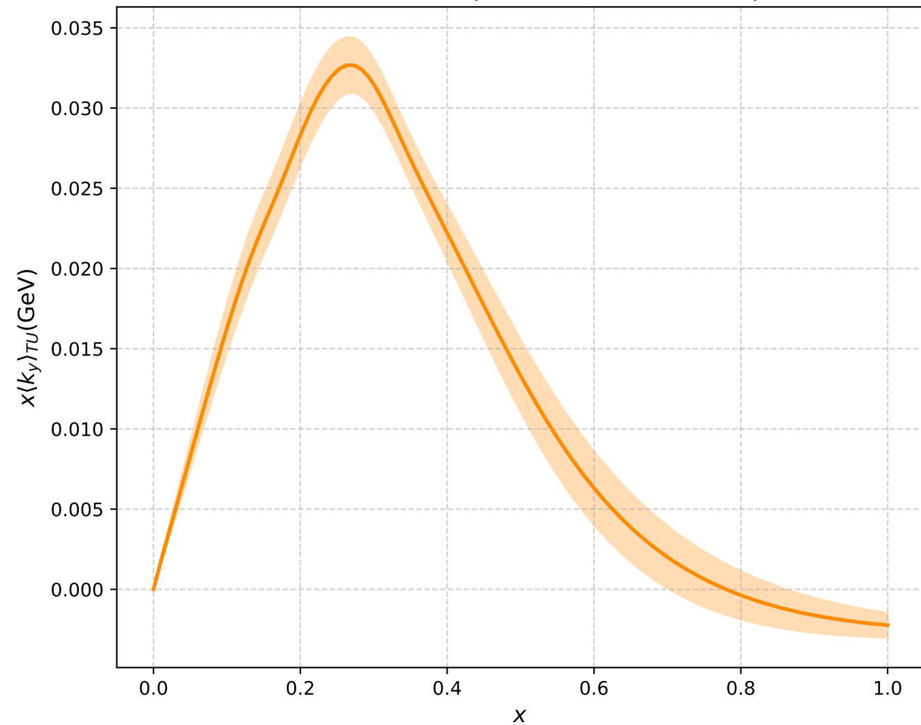
x^* Sivers Shift (\hat{\zeta} \rightarrow \infty, b^2=9.0) [c + d/\hat{\zeta}^2]
