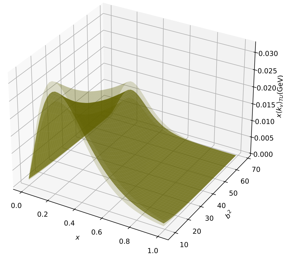
x\langle k_y \rangle_{TU}(\text{GeV}) (P_L=-3)
