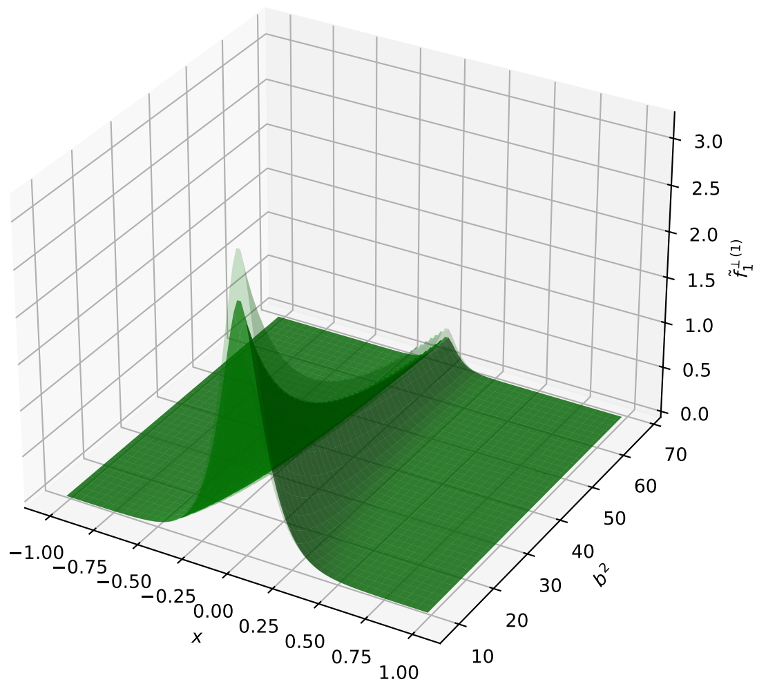
\tilde{f}_1^{\perp(1)} = -2\tilde{A}_{12B} (P_L=-3)
