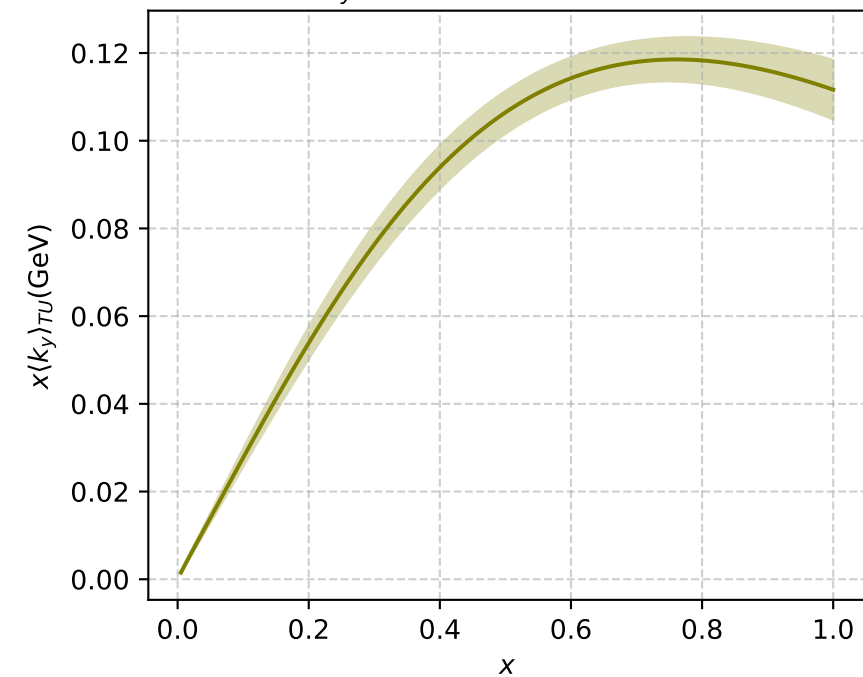
x\langle k_y \rangle_{TU}(\text{GeV}) (P_L=-1, b^2=9)
