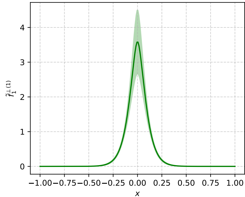
\tilde{f}_1^{\perp(1)} = -2\tilde{A}_{12B} (\hat{\zeta} \rightarrow \infty, b^2=9.0) [c + d/\hat{\zeta}^2]
