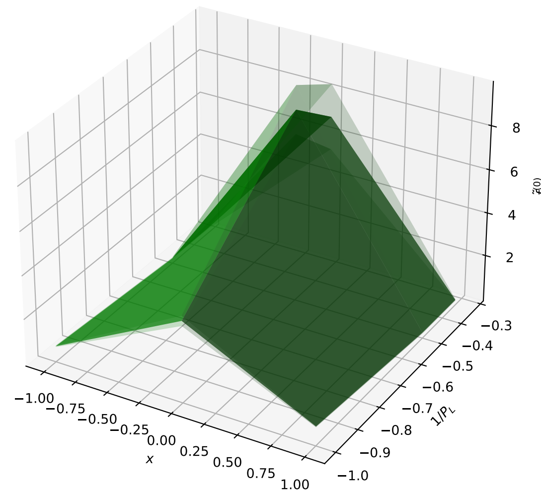
x\langle k_y \rangle_{TU}(\text{GeV}) (b^2=9.0)
