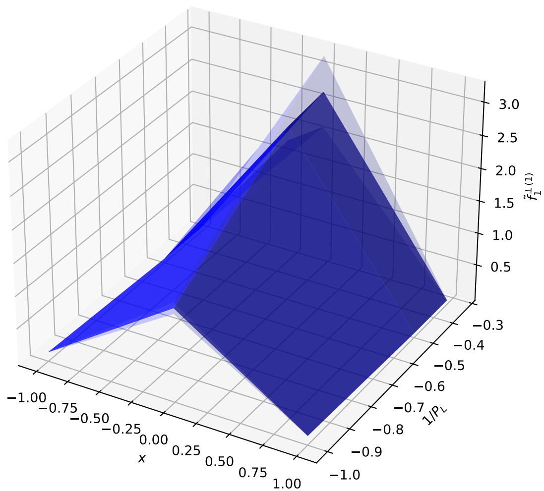
\tilde{f}_1^{\perp(1)} = -2\tilde{A}_{12B} (b^2=9.0)
