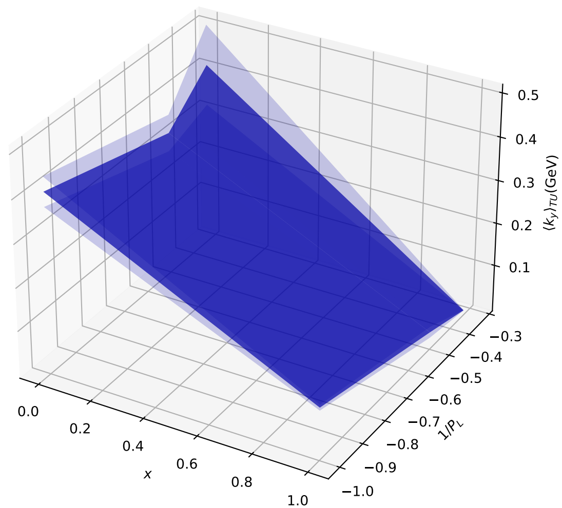
\langle k_y \rangle_{TU}(\text{GeV}) (b^2=9.0)
