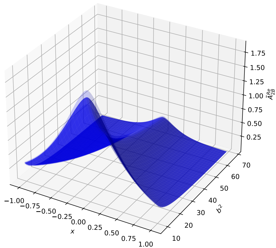
\tilde{f}_1^{\perp(1)} = -2\tilde{A}_{12B} (P_L=-1)
