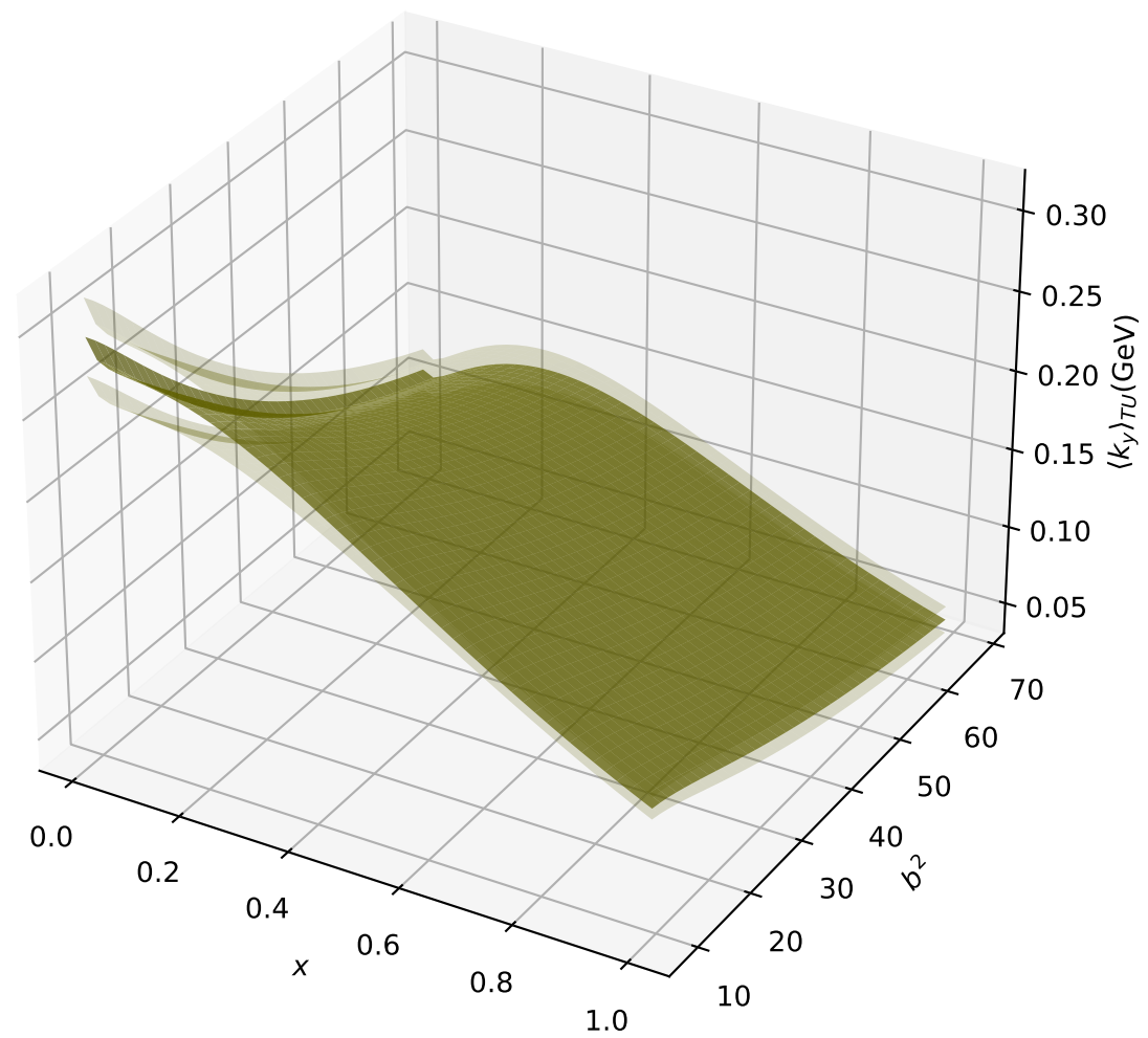
\langle k_y \rangle_{TU}(\text{GeV}) (P_L=-1)
