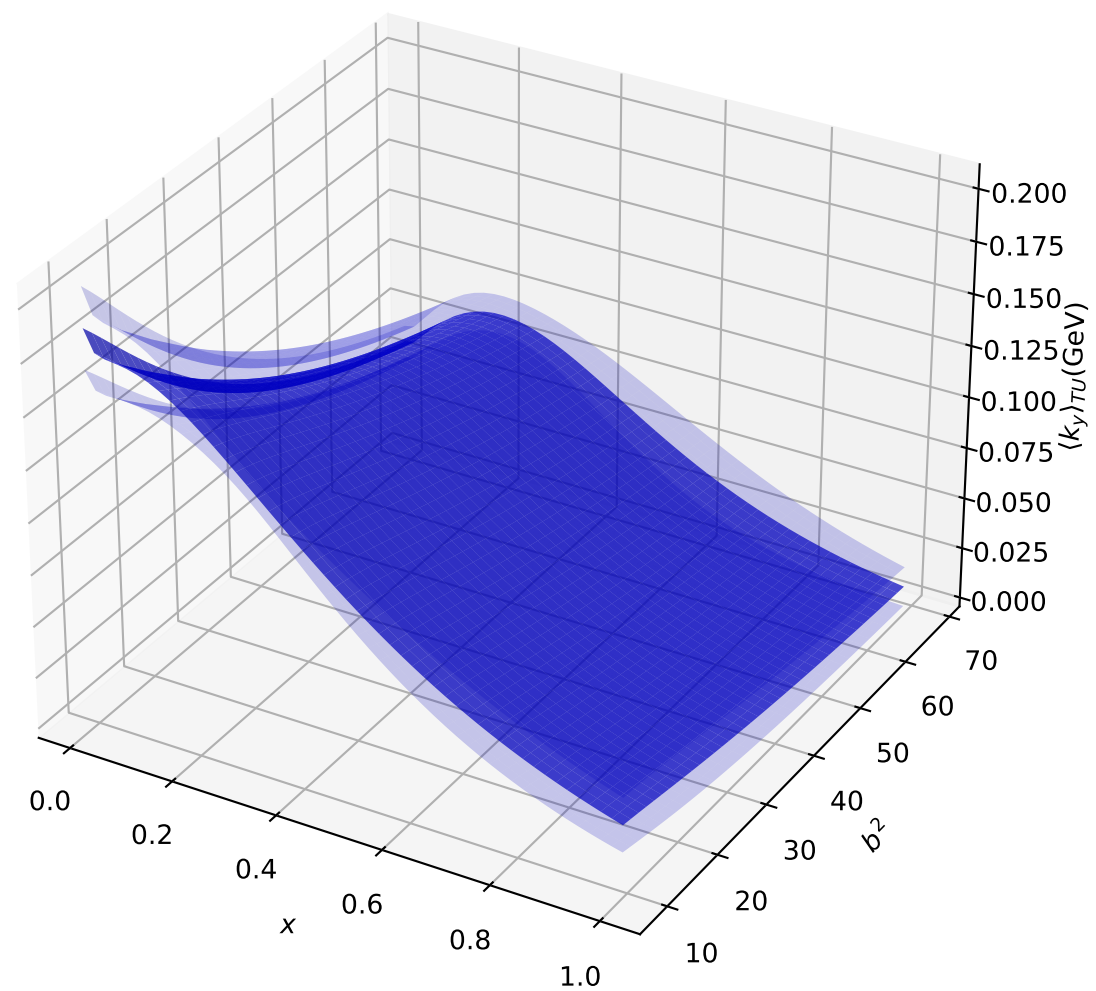
\langle k_y \rangle_{TU}(\text{GeV}) (P_L=-2)
