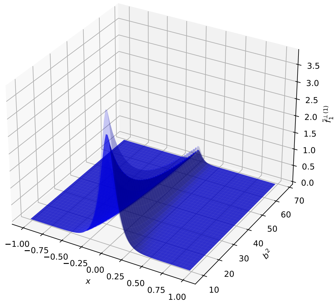
\tilde{f}_1^{\perp(1)} = -2\tilde{A}_{12B} (P_L=-4)
