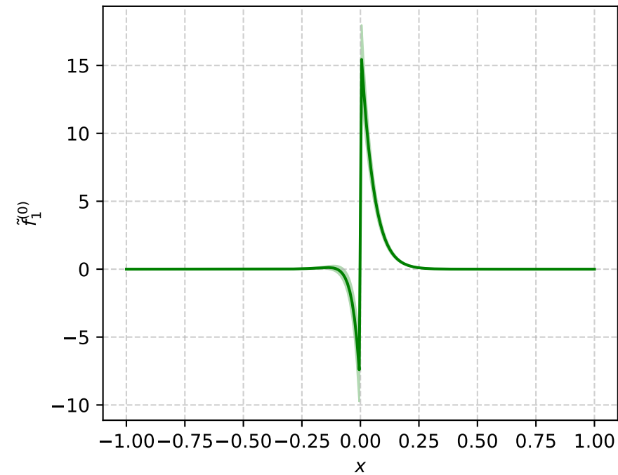
\tilde{f}_1^{(0)} = 2\tilde{A}_{2B} (P_L=-4, b^2=36)
