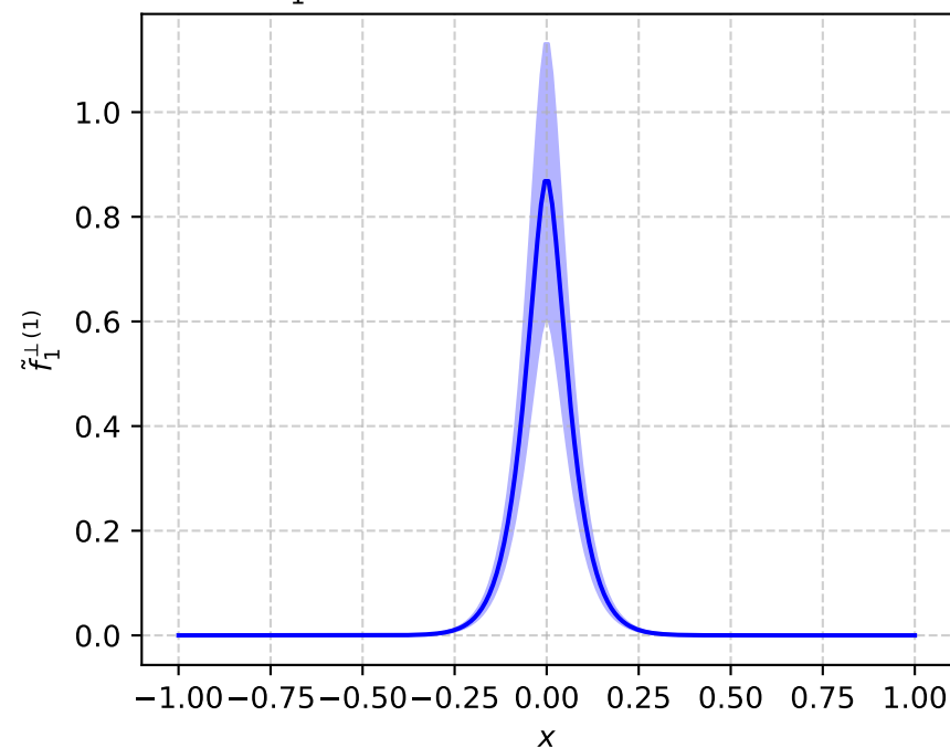
\tilde{f}_1^{\perp(1)} = -2\tilde{A}_{12B} (P_L=-4, b^2=36)
