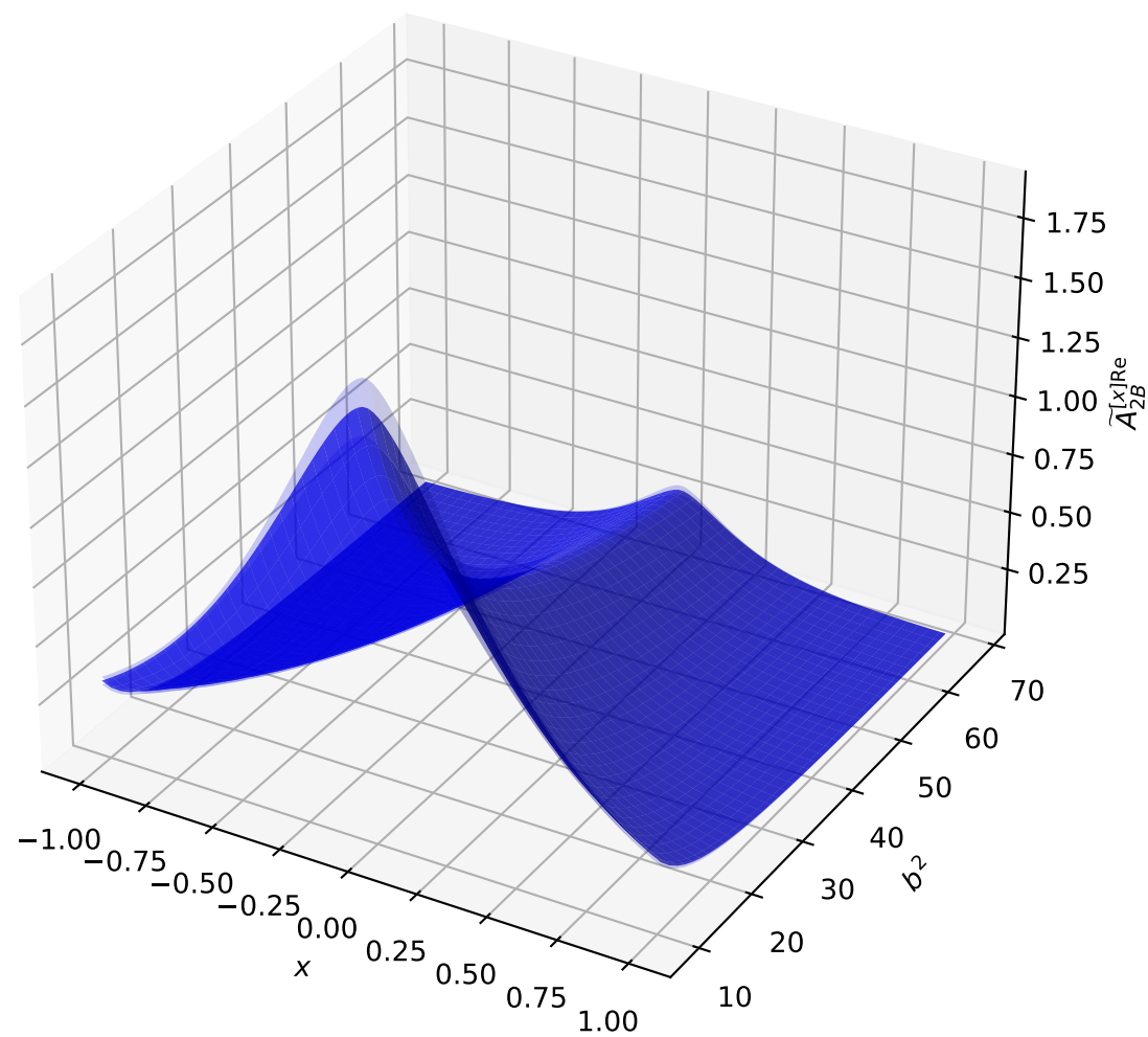
\widetilde{f}_{1T}^{\perp(1)} = -2\widetilde{A}_{12B}^{[x]\text{Re}} (P_L=-1)
