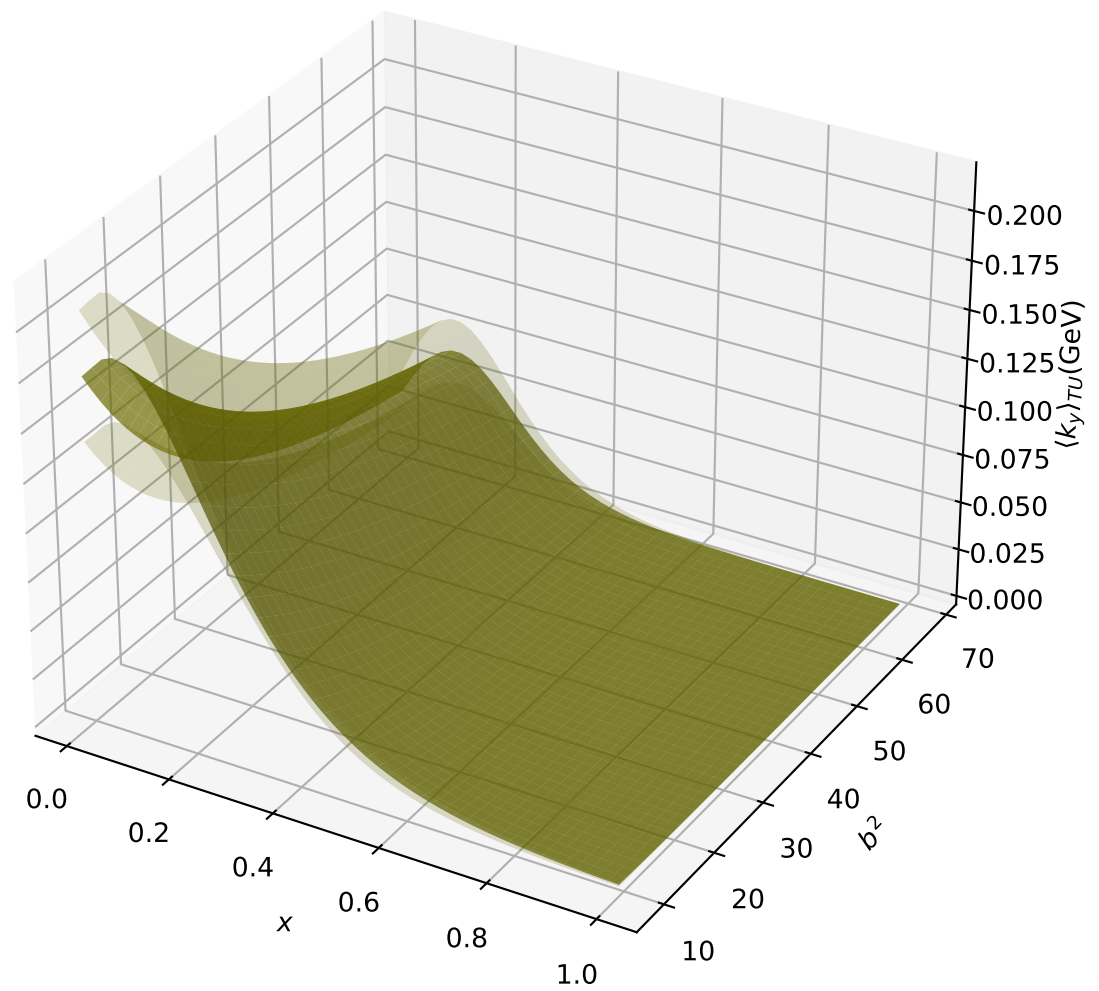
\langle k_y \rangle_{TU}(\text{GeV}) (P_L=-3)
