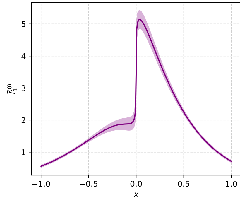
\tilde{f}_1^{(0)} = 2\widetilde{A}_{2B}^{[x]} (P_L=-1, b^2=9)
