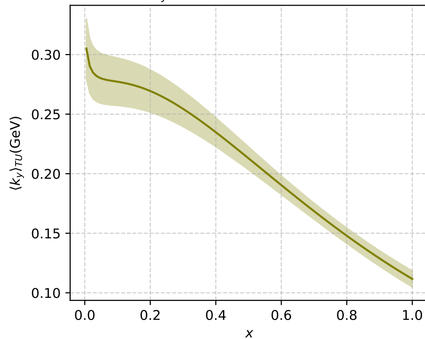
\langle k_y \rangle_{TU}(\text{GeV}) (P_L=-1, b^2=9)
