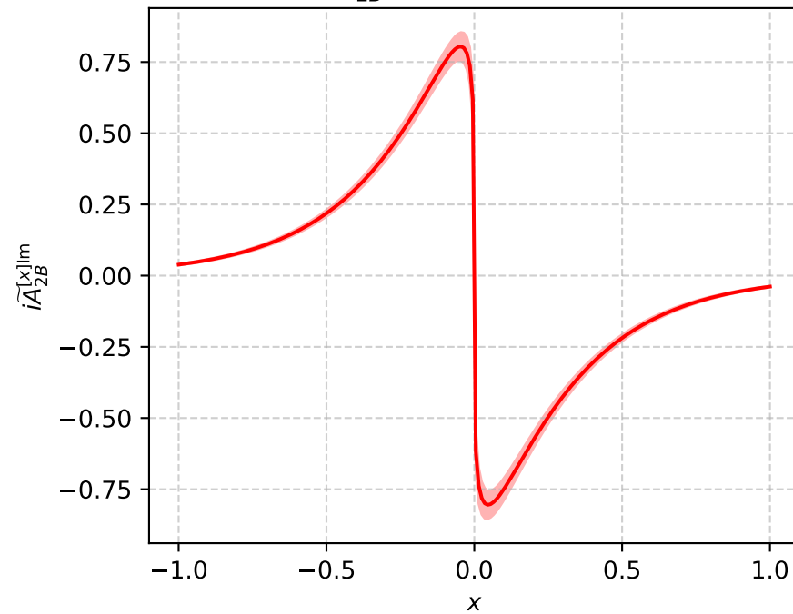
i\widetilde{A}_{2B}^{[x]\text{Im}} (P_L=-1, b^2=9)
