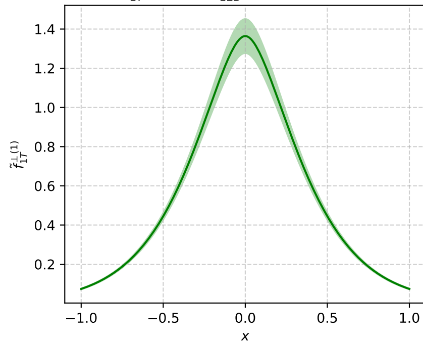
\tilde{f}_{1T}^{(1)} = -2\widetilde{A}_{12B}^{[x]\text{Re}} (P_L=-1, b^2=9)
