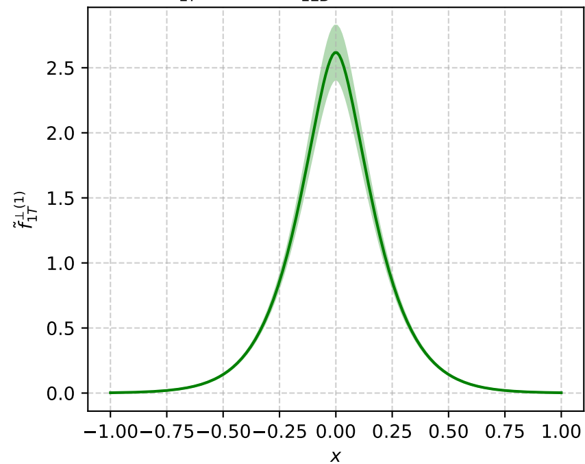
\check{f}_{1T}^{\perp(1)} = -2\widetilde{A}_{12B}^{[x]\text{Re}} (P_L=-2, b^2=9)
