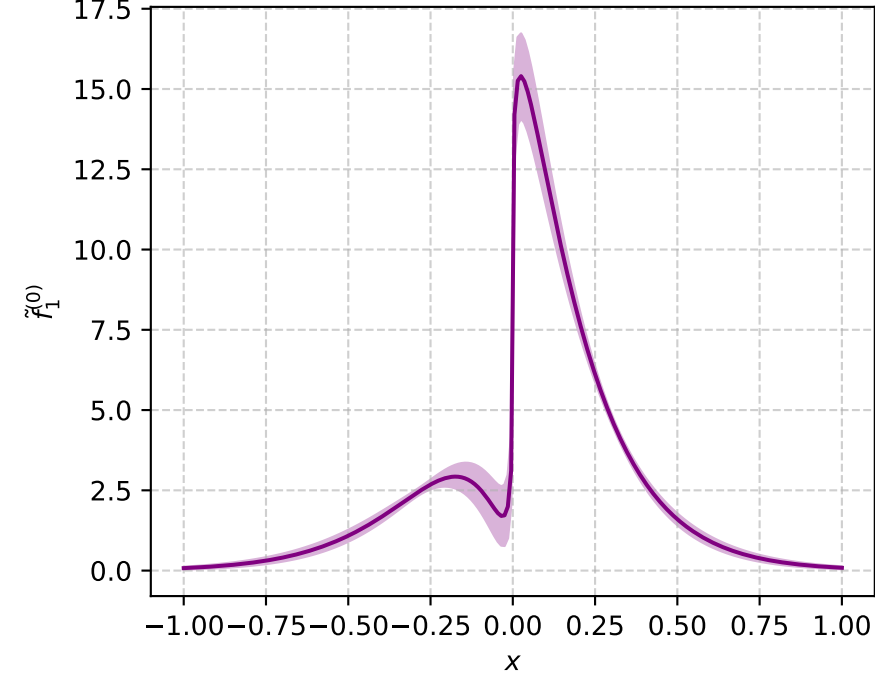
\check{f}_1^{(0)} = 2\widetilde{A}_{2B}^{[x]} (P_L=-2, b^2=9)
