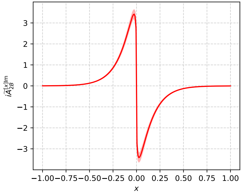
i\widetilde{A}_{2B}^{[x]\text{Im}} (P_L=-2, b^2=9)
