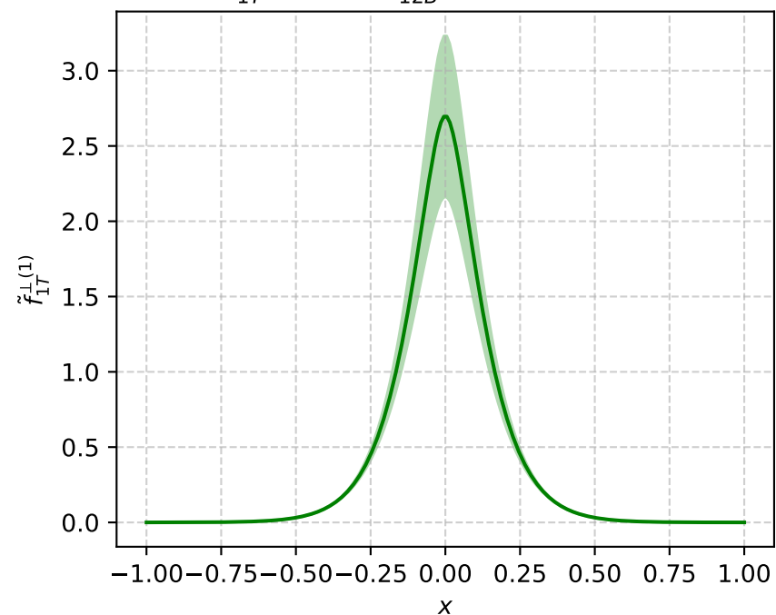
\check{f}_{1T}^{\perp(1)} = -2\widetilde{A}_{12B}^{[x]\text{Re}} (P_L=-3, b^2=9)
