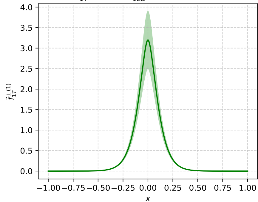
\widetilde{f}_{1T}^{\perp(1)} = -2\widetilde{A}_{12B}^{[x]\text{Re}} (P_L=-4, b^2=9)
