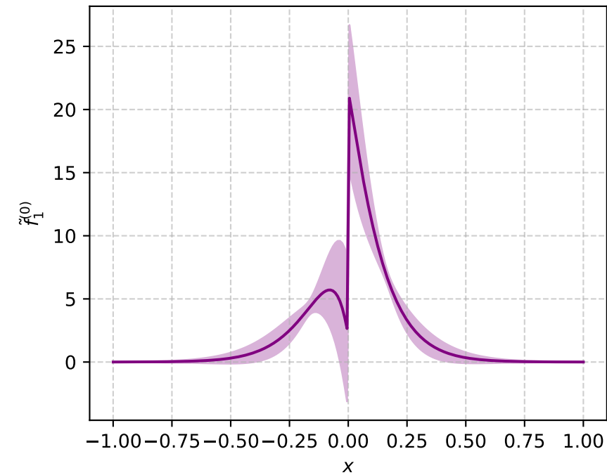
\widetilde{f}_1^{(0)} = 2\widetilde{A}_{2B}^{[x]} (P_L=-4, b^2=9)
