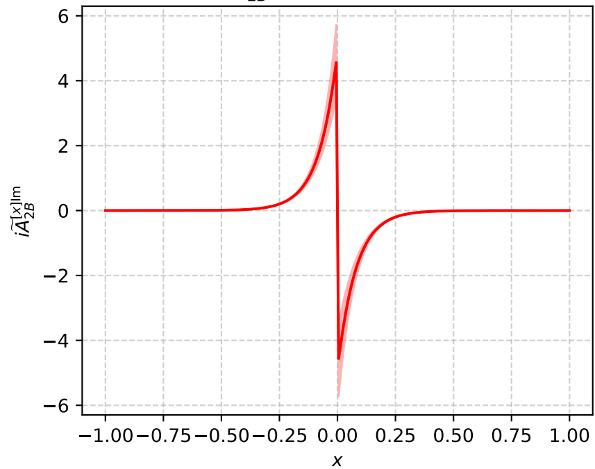
i\widetilde{A}_{2B}^{[x]\text{Im}} (P_L=-4, b^2=9)
