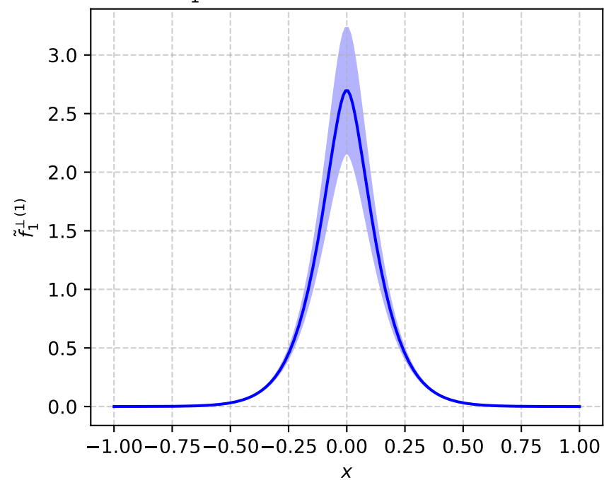
\tilde{f}_1^{(1)} = -2\tilde{A}_{12B} (P_L=-3, b^2=9)
