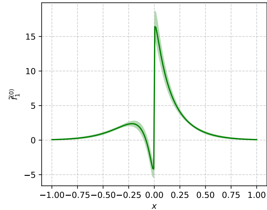
\tilde{f}_1^{(0)} = 2\tilde{A}_{2B} (P_L=-3, b^2=9)
