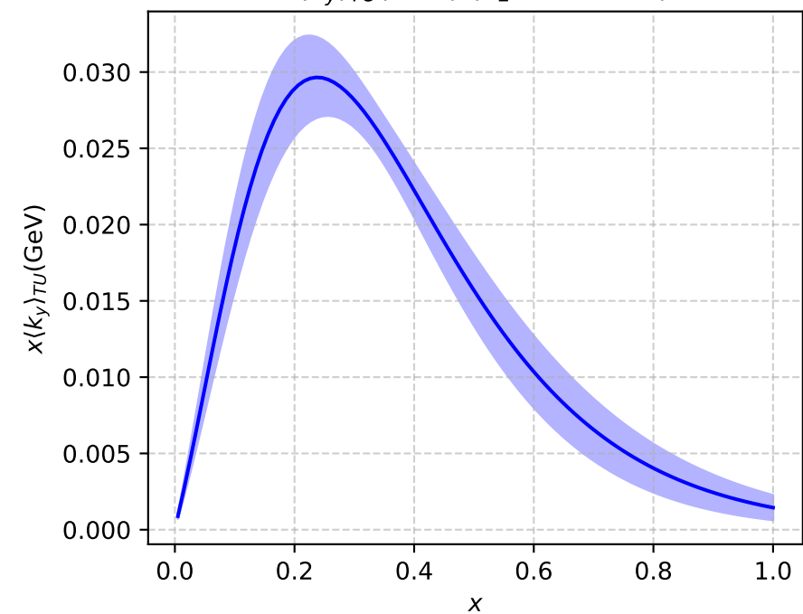
x\langle k_y \rangle_{TU}(\text{GeV}) (P_L=-3, b^2=9)
