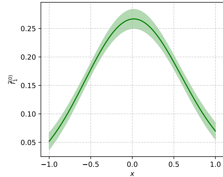
\tilde{f}_1^{(0)} = 2\tilde{A}_{2B} (P_L=-1, b^2=50)
