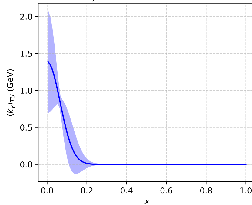
\langle k_y \rangle_{TU} \text{ (GeV)} (P_L=-2, b^2=9)
