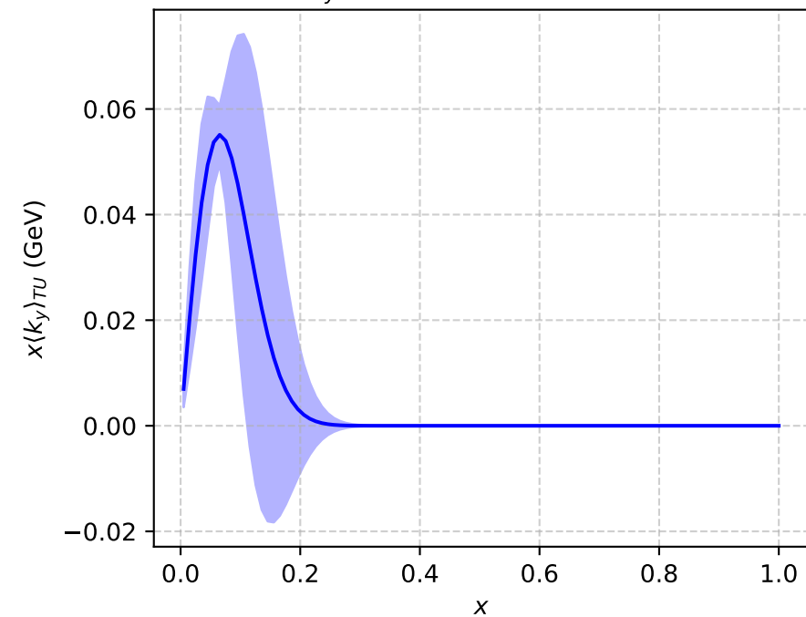
x\langle k_y \rangle_{TU} \text{ (GeV)} (P_L=-2, b^2=9)
