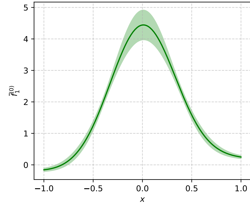
\tilde{f}_1^{(0)} = 2\tilde{A}_{2B} (P_L=-2, b^2=9)
