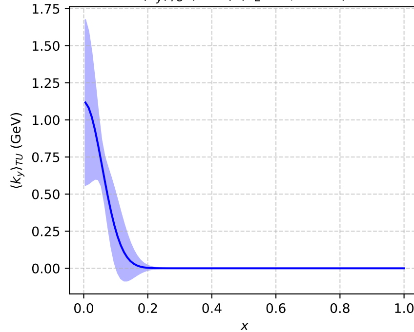
\langle k_y \rangle_{TU} \text{ (GeV)} (P_L=-3, b^2=9)
