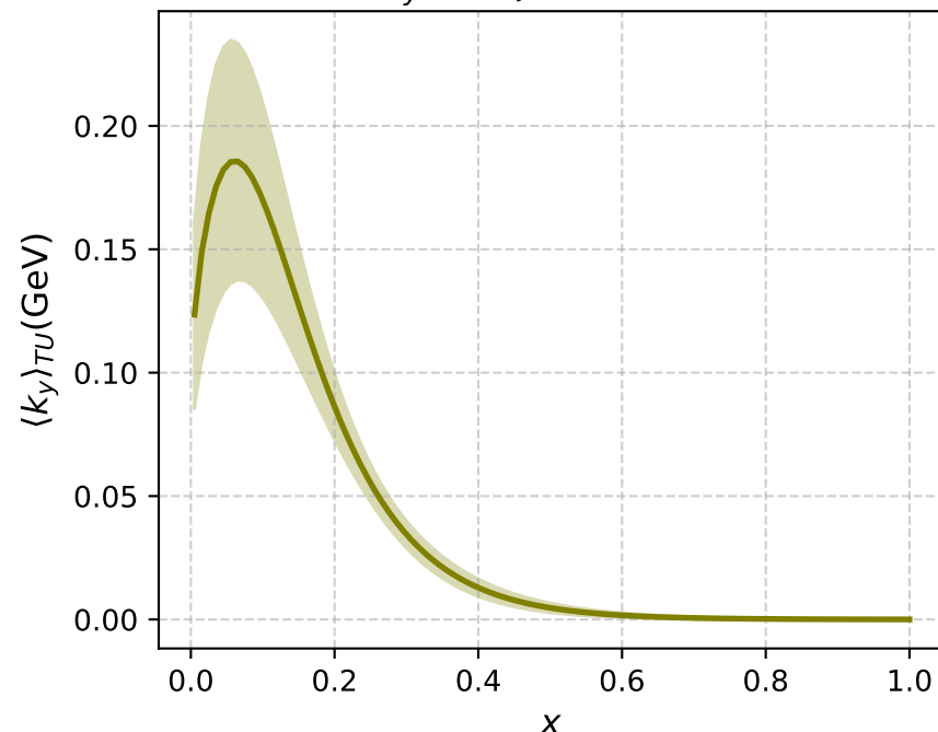
\text{Sivers Shift } \langle k_y \rangle_{TU} (\hat{\zeta} \rightarrow \infty, b^2=9.0) [c + d/\hat{\zeta}]
