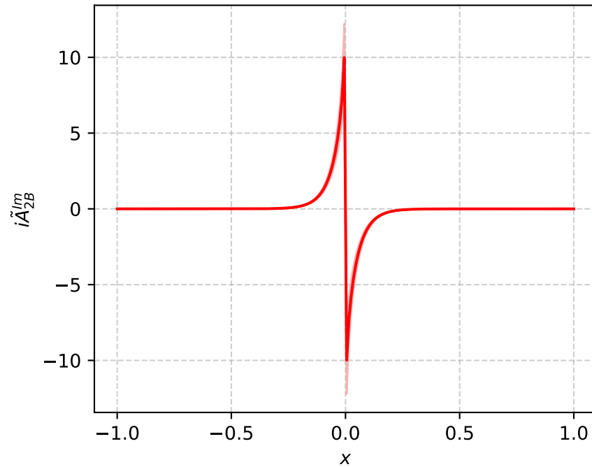
i\tilde{A}_{2B}^{Im} (\hat{\zeta} \rightarrow \infty, b^2=9.0) [c + d/\hat{\zeta}]
