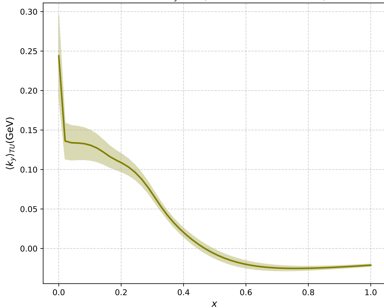
Sivers Shift \langle k_y \rangle_{TU} (\hat{\zeta} \rightarrow \infty, b^2=9.0) [c + d/\hat{\zeta}]
