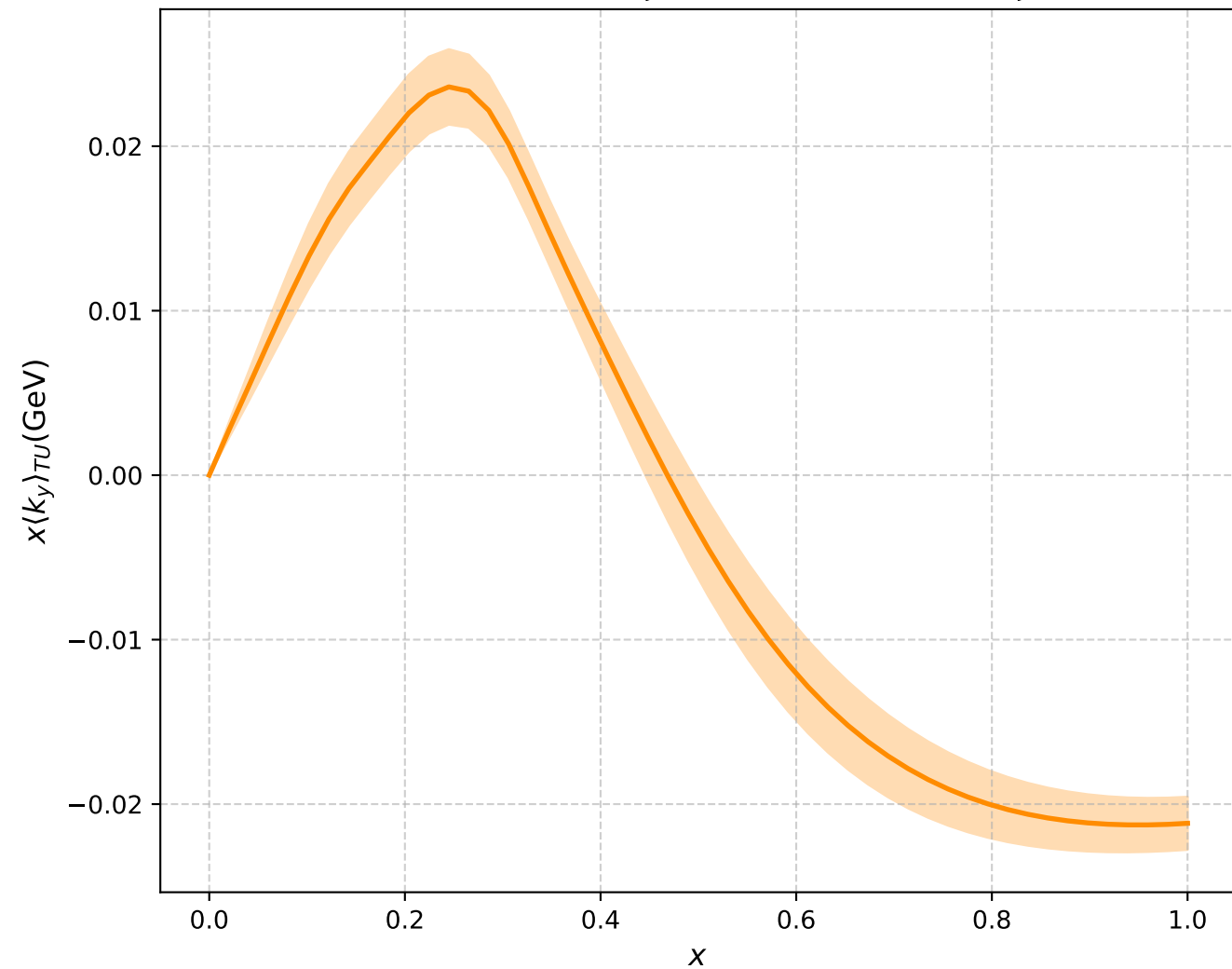
x^* Sivers Shift \langle k_y \rangle_{TU} (\hat{\zeta} \rightarrow \infty, b^2=9.0) [c + d/\hat{\zeta}]
