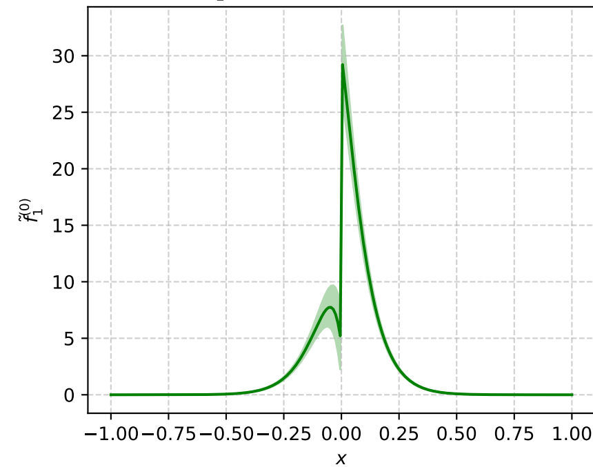
\tilde{f}_1^{(0)} = 2\tilde{A}_{2B} (P_L=-4, b^2=9)
