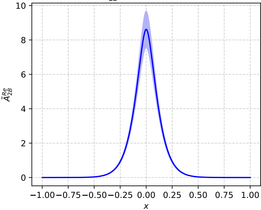
\tilde{f}_1^{\perp(1)} = -2\tilde{A}_{12B} (P_L=-4, b^2=9)
