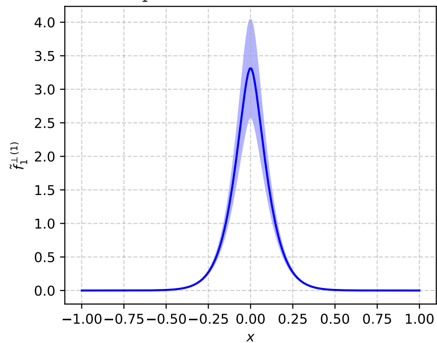
\tilde{f}_1^{\perp(1)} = -2\tilde{A}_{12B} (P_L=-4, b^2=9)
