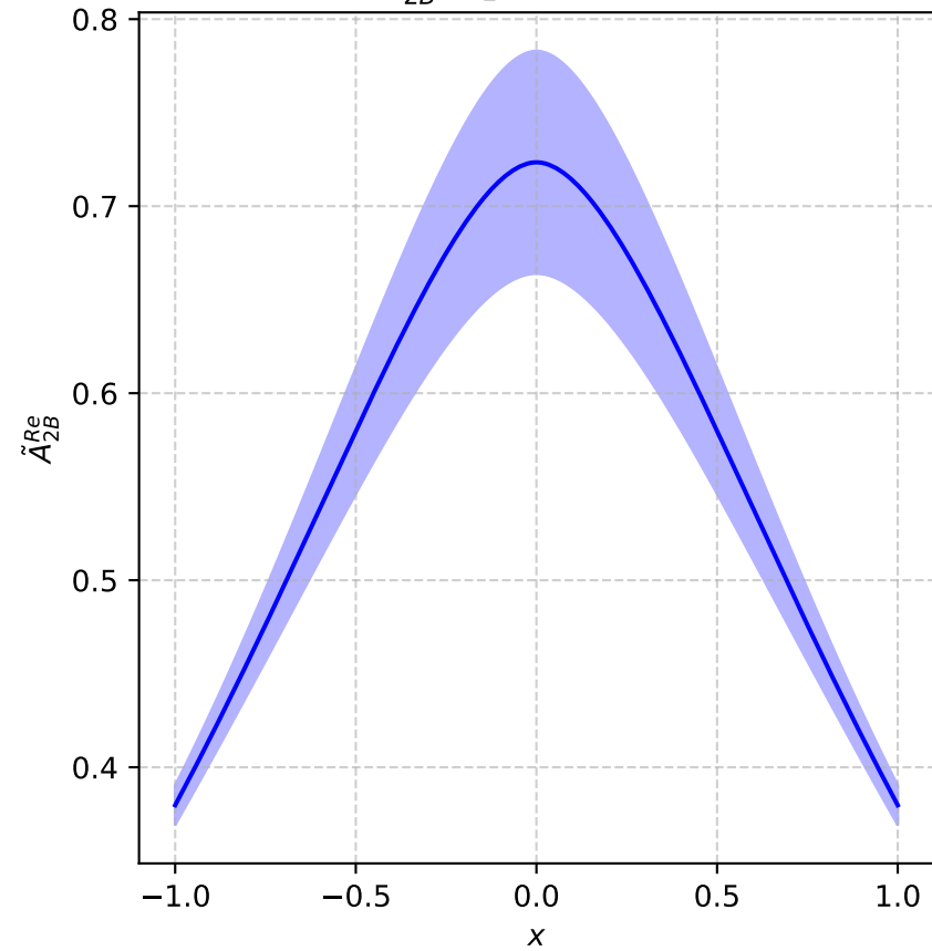
\tilde{A}_{2B}^{Re} (P_L=-1, b^2=9)
