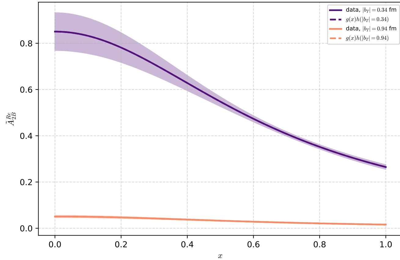
Gaussian(P.b) - Exp(bT)
