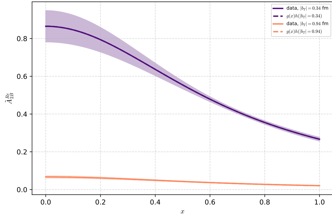
Gaussian(P.b) - PowerLaw(bT)
