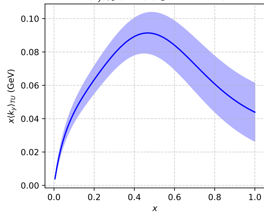
x\langle k_y \rangle_{TU} \text{ (GeV)} (P_L=-1, b^2=50)
