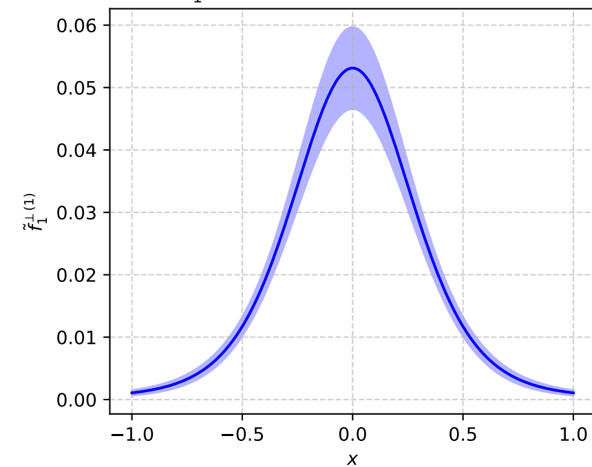
\tilde{f}_1^{\perp(1)} = -2\tilde{A}_{12B} (P_L=-1, b^2=50)
