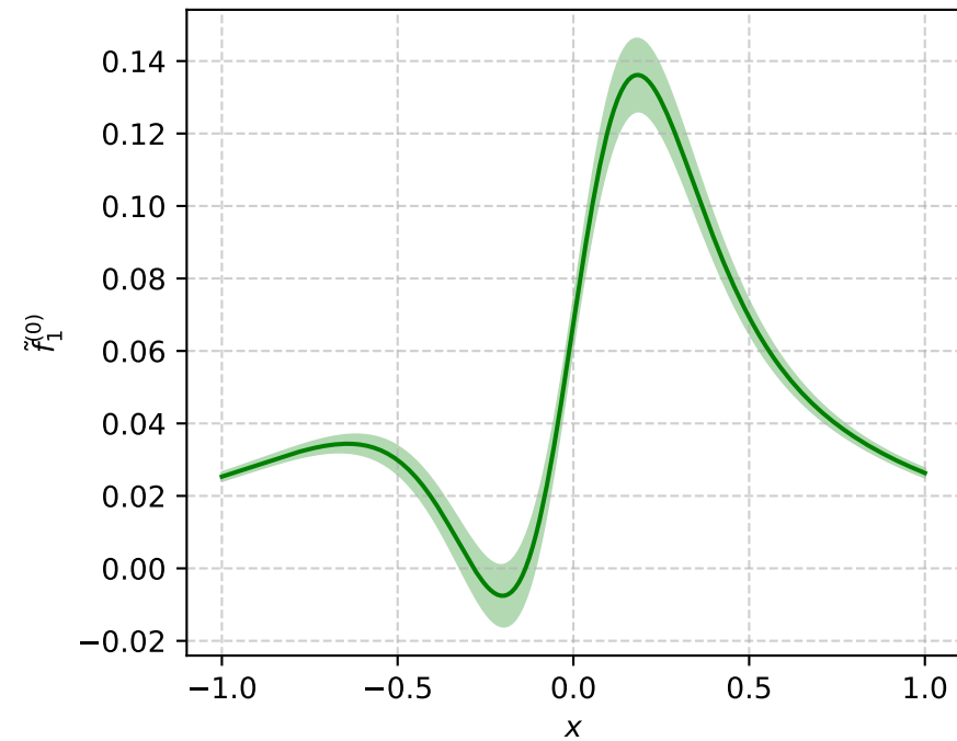
\tilde{f}_1^{(0)} = 2\tilde{A}_{2B} (P_L=-1, b^2=50)
