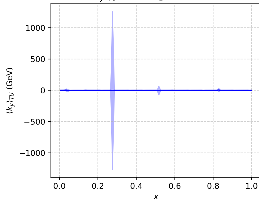
\langle k_y \rangle_{TU} \text{ (GeV)} (P_L=-4, b^2=36)
