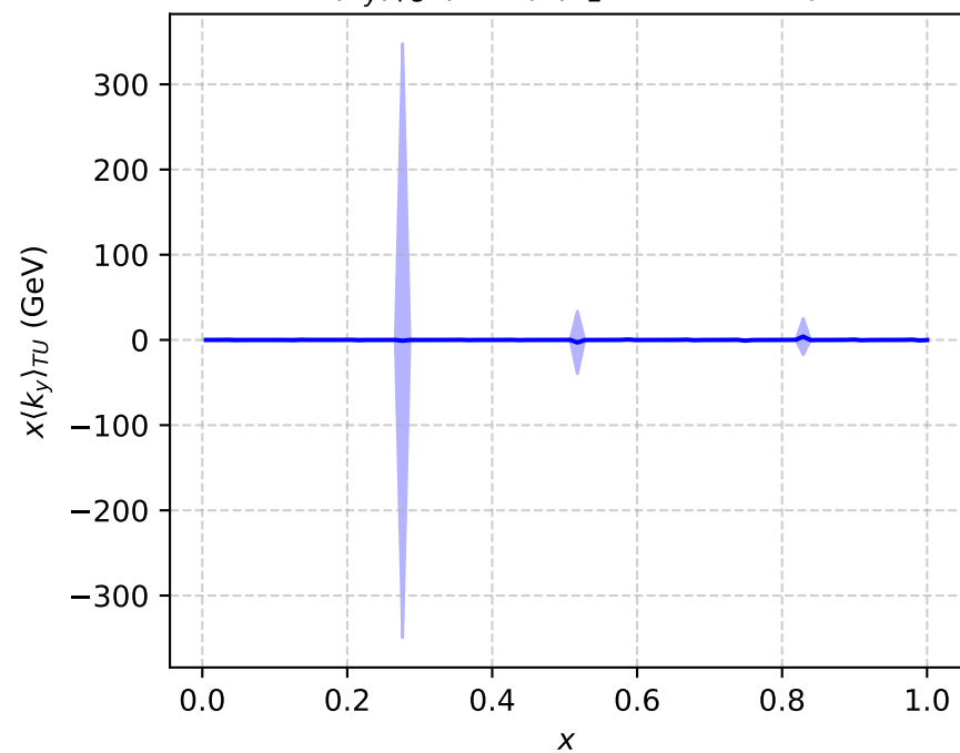
x\langle k_y \rangle_{TU} \text{ (GeV)} (P_L=-4, b^2=36)
