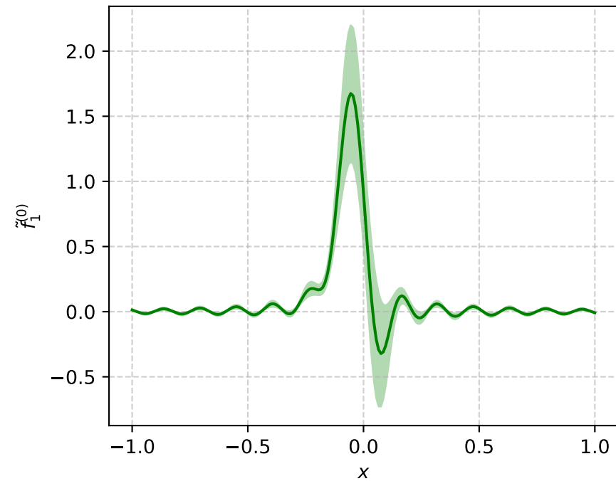
\tilde{f}_1^{(0)} = 2\tilde{A}_{2B} (P_L=-4, b^2=36)
