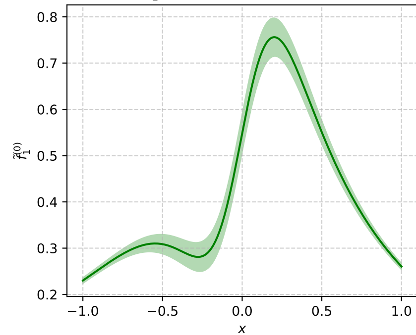
\tilde{f}_1^{(0)} = 2\tilde{A}_{2B} (P_L=-1, b^2=9)
