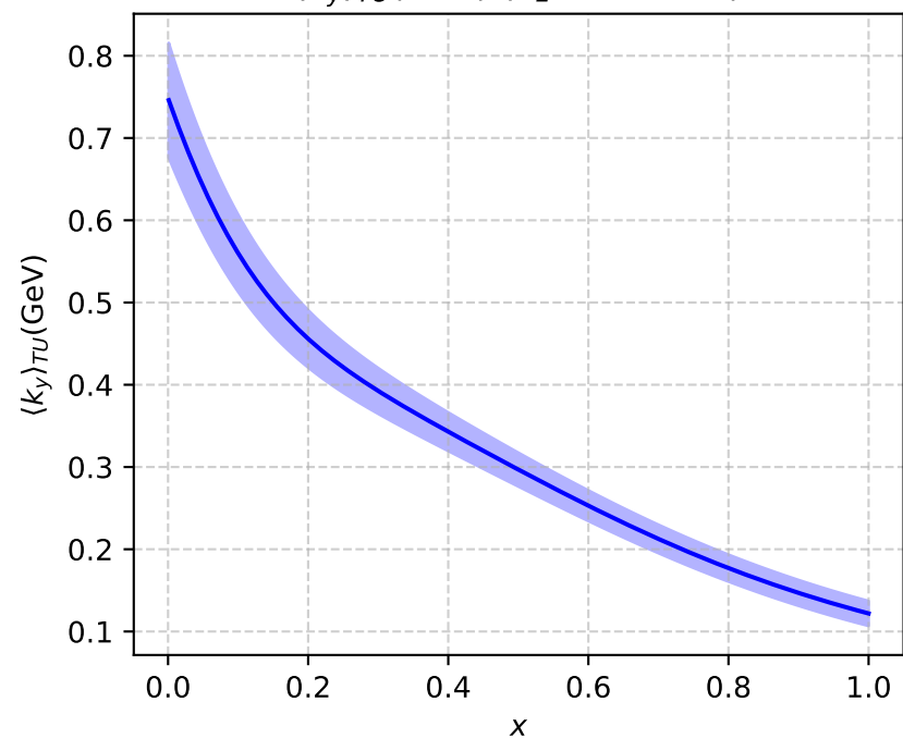
\langle k_y \rangle_{TU}(\text{GeV}) (P_L=-1, b^2=9)
