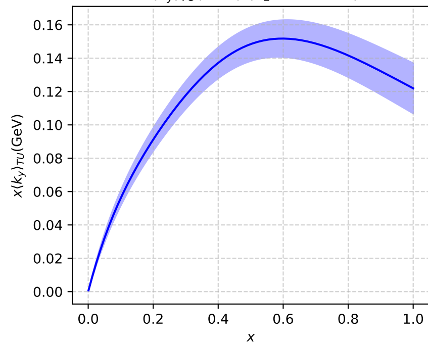
x\langle k_y \rangle_{TU}(\text{GeV}) (P_L=-1, b^2=9)
