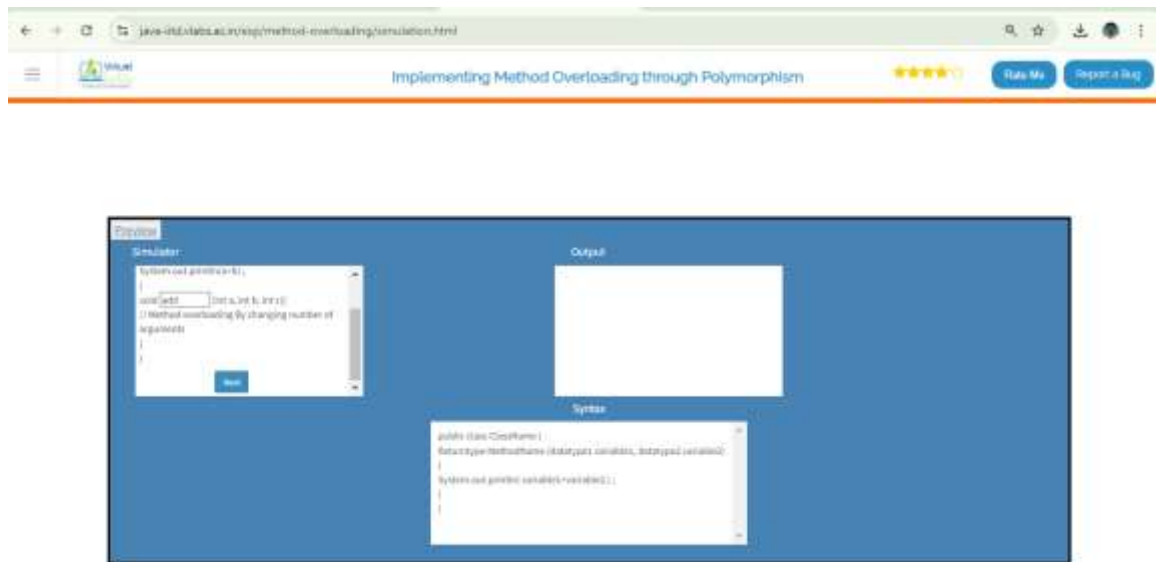
Fig:2 Simulation on method overloading
