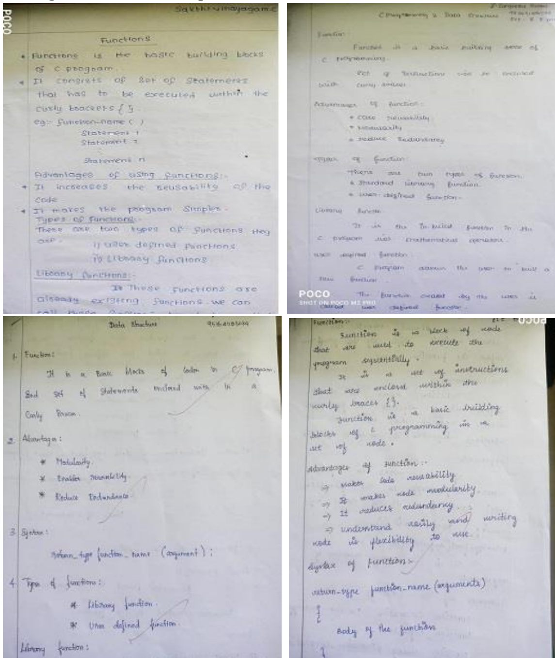
Figure 1: Minute Paper
