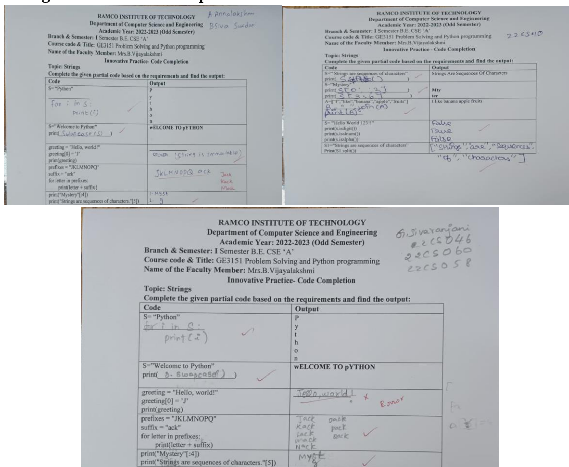
Fig 1: Sample Questions
