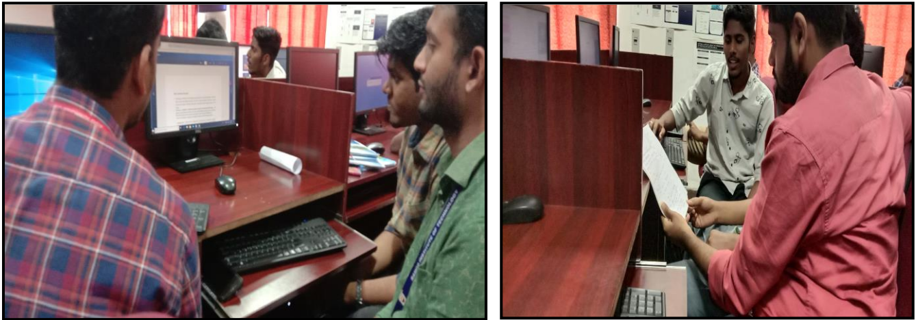
Fig.1. Idea Discussion
