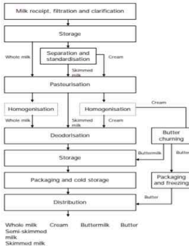
Figure 1.Flowchart showing Milk and milk product Processing
