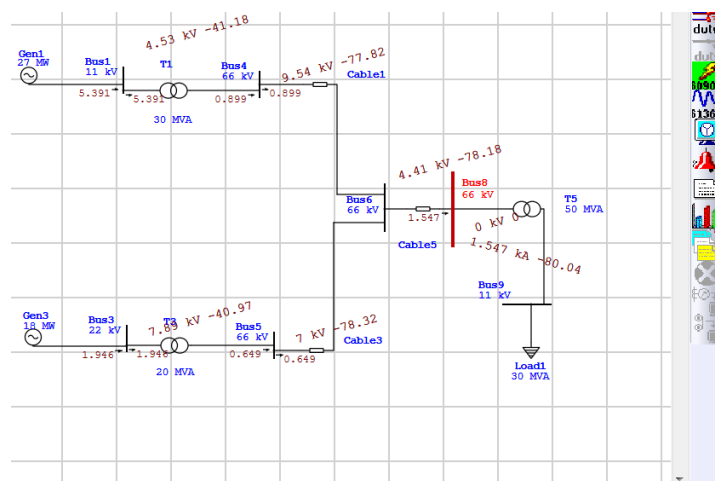
After Fault
