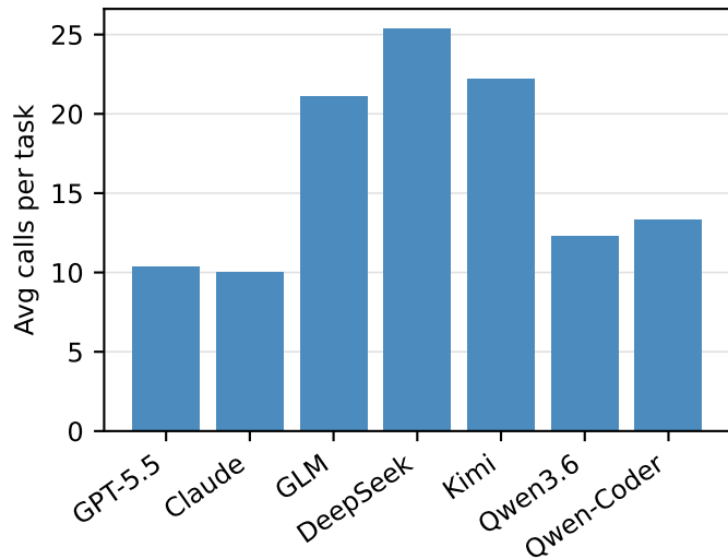
Schema exploration
