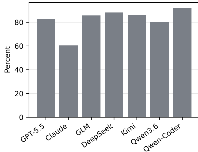
Navigation-trap rate
