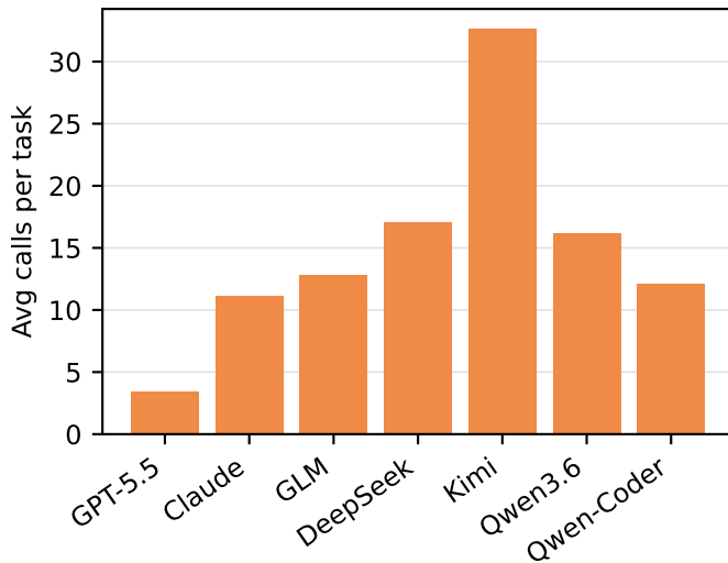
Execution attempts
