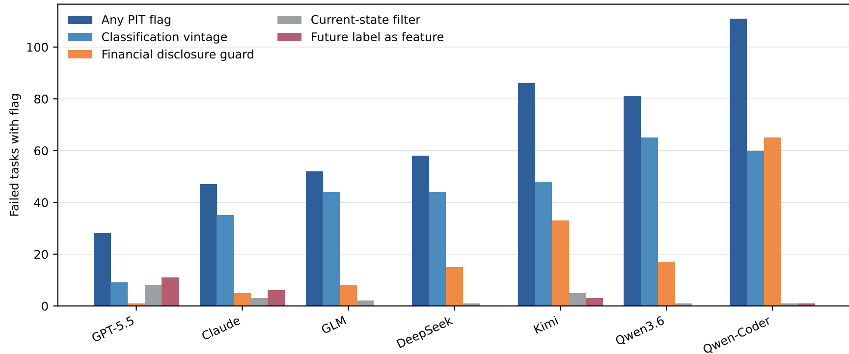
Point-in-time diagnostic flags by model
