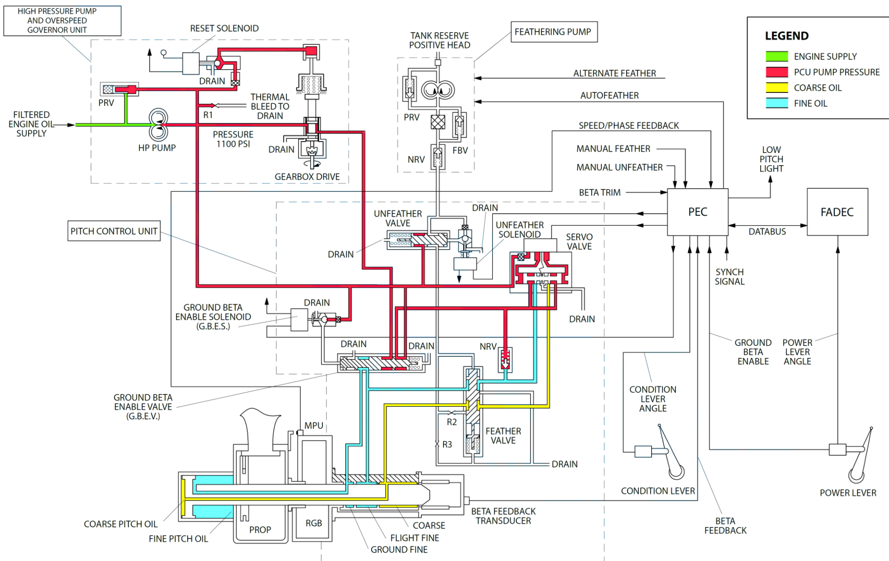
Figure 61-19 Maximum Reverse
