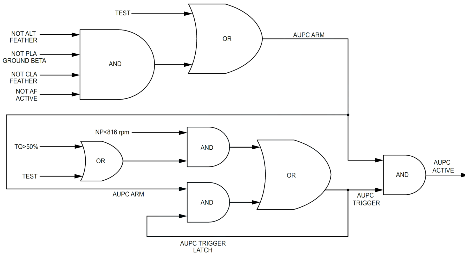
Figure 61-23 AUPC Logic
