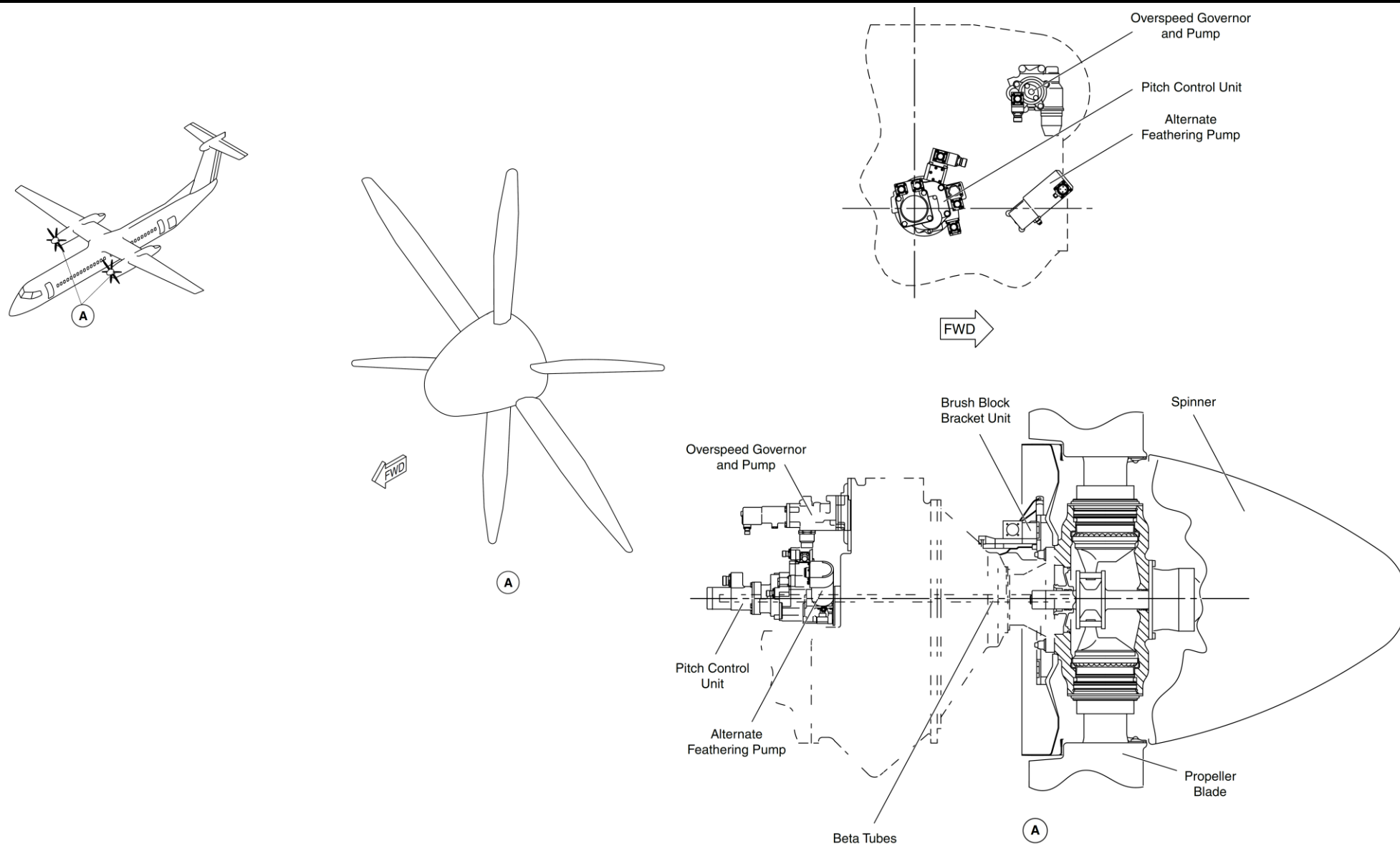
Figure 61-1 Propeller Assembly
