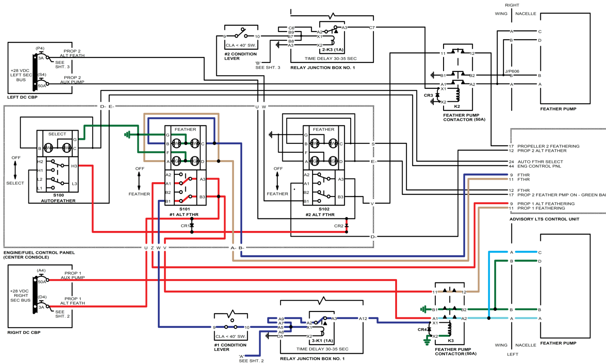
Figure 61-41 Alternate Feather
