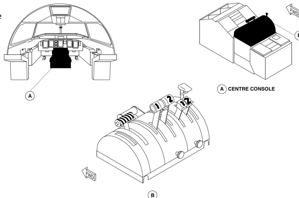
Figure 61-11 Power Quadrant
