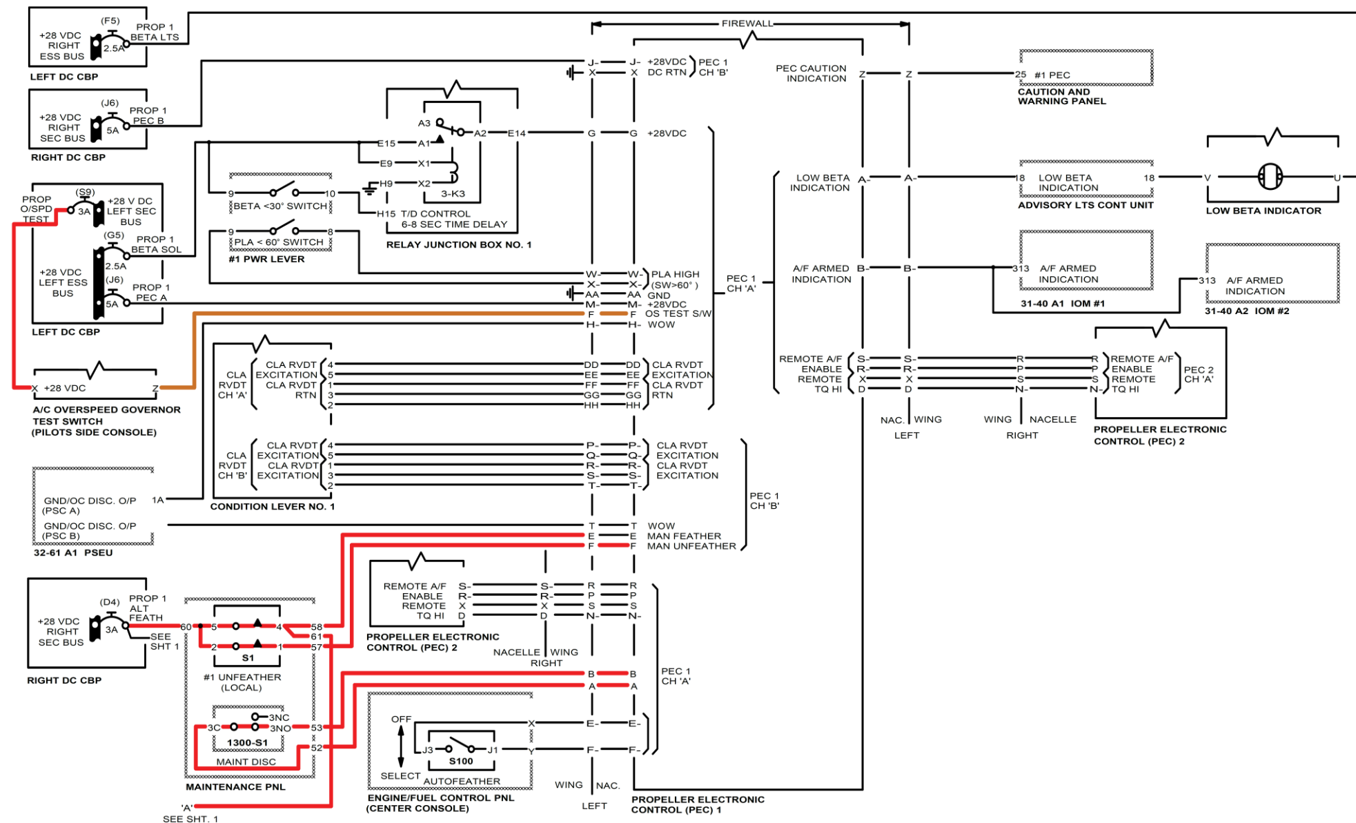
Figure 61-42 Propeller Overspeed Governor Test (Sheet 1 of 2)
