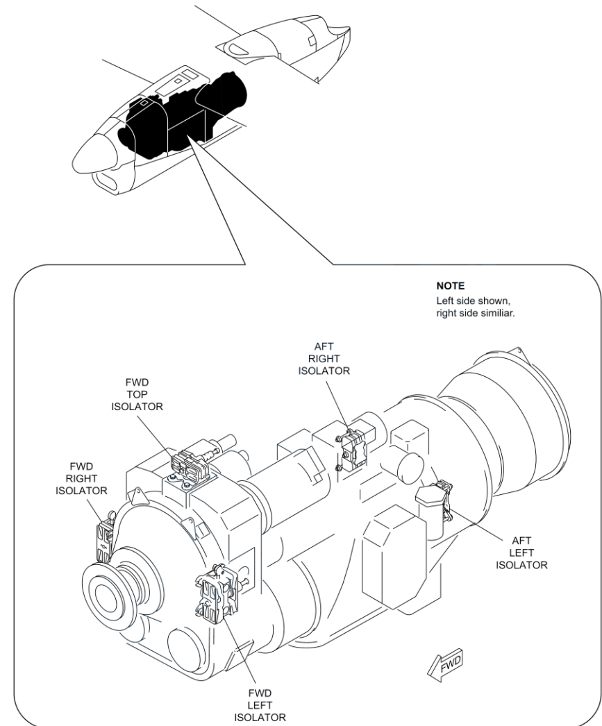
Figure 71-6A Engine Vibration Isolation System
