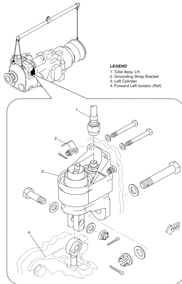
Figure 71-12 Cylinder Assembly
