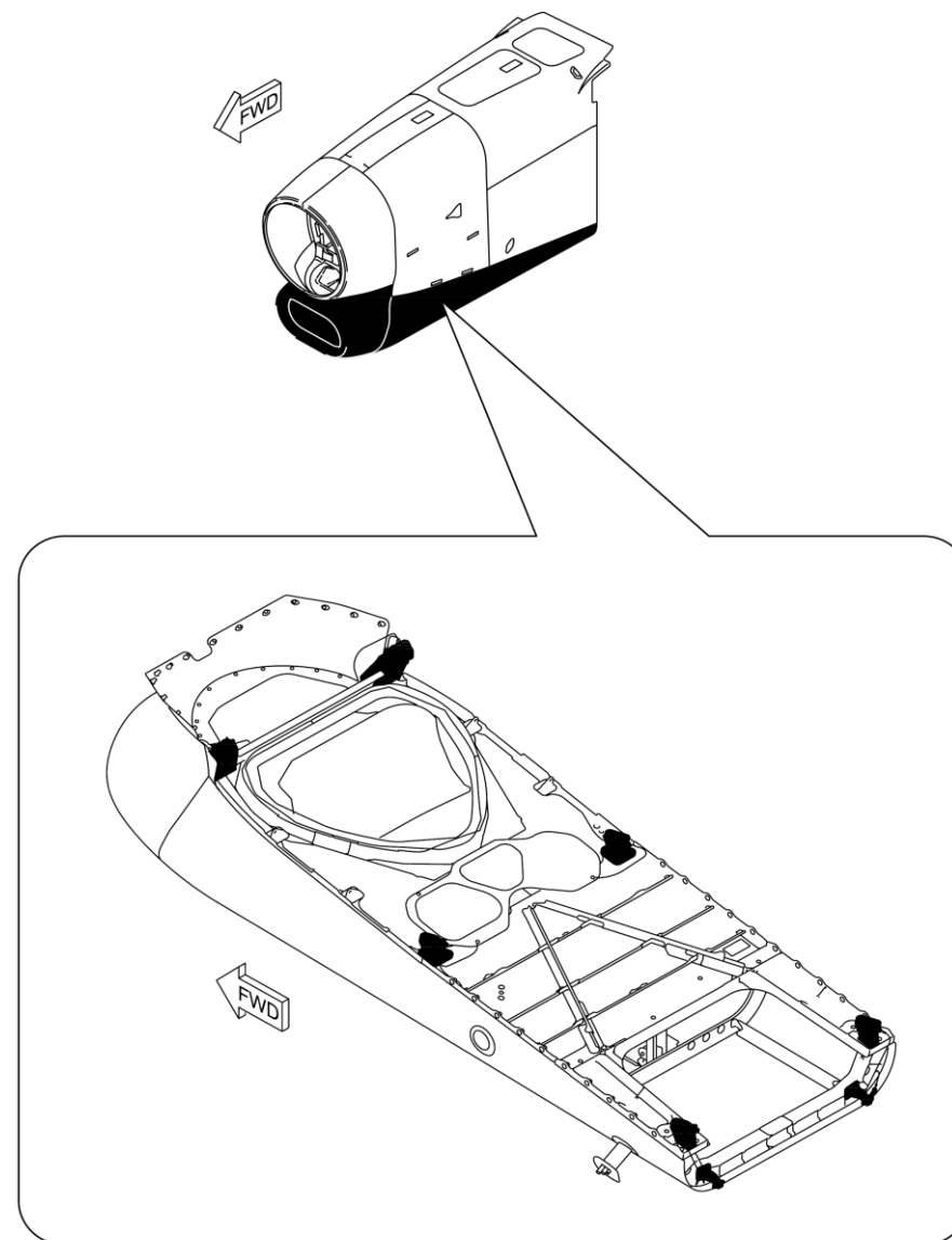
Figure 71-4 Lower Cowl
