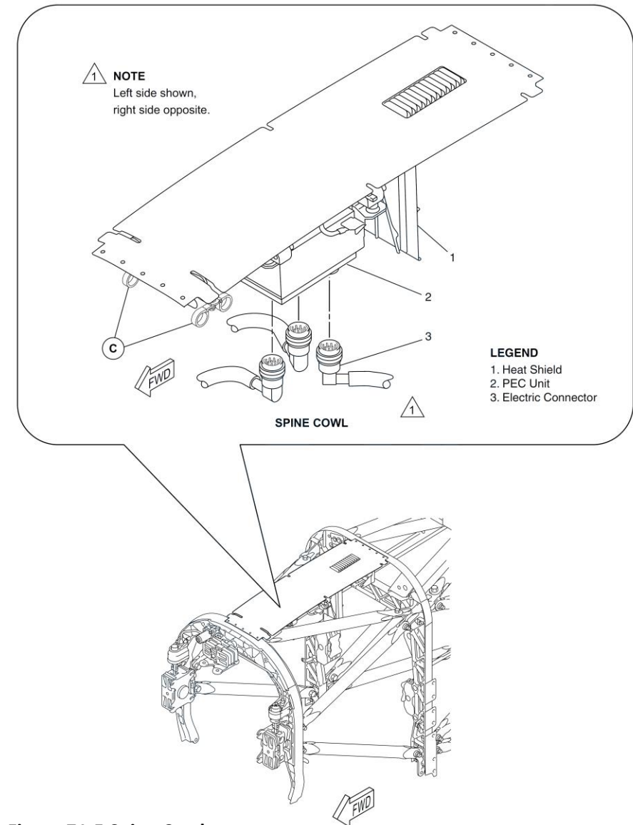
Figure 71-5 Spine Cowl
