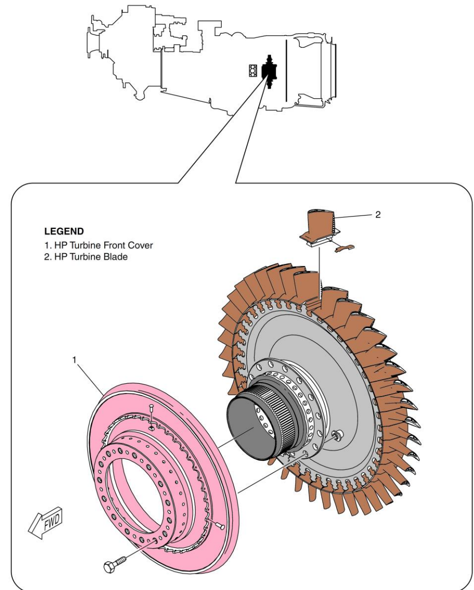
Figure 72-16 High Pressure Turbine
