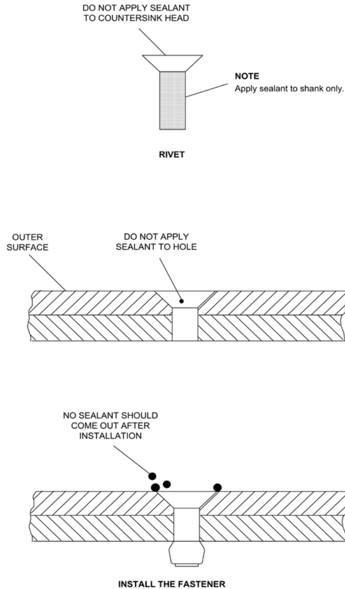
Figure 51-8 Wet Installation of Permanent Fasteners
