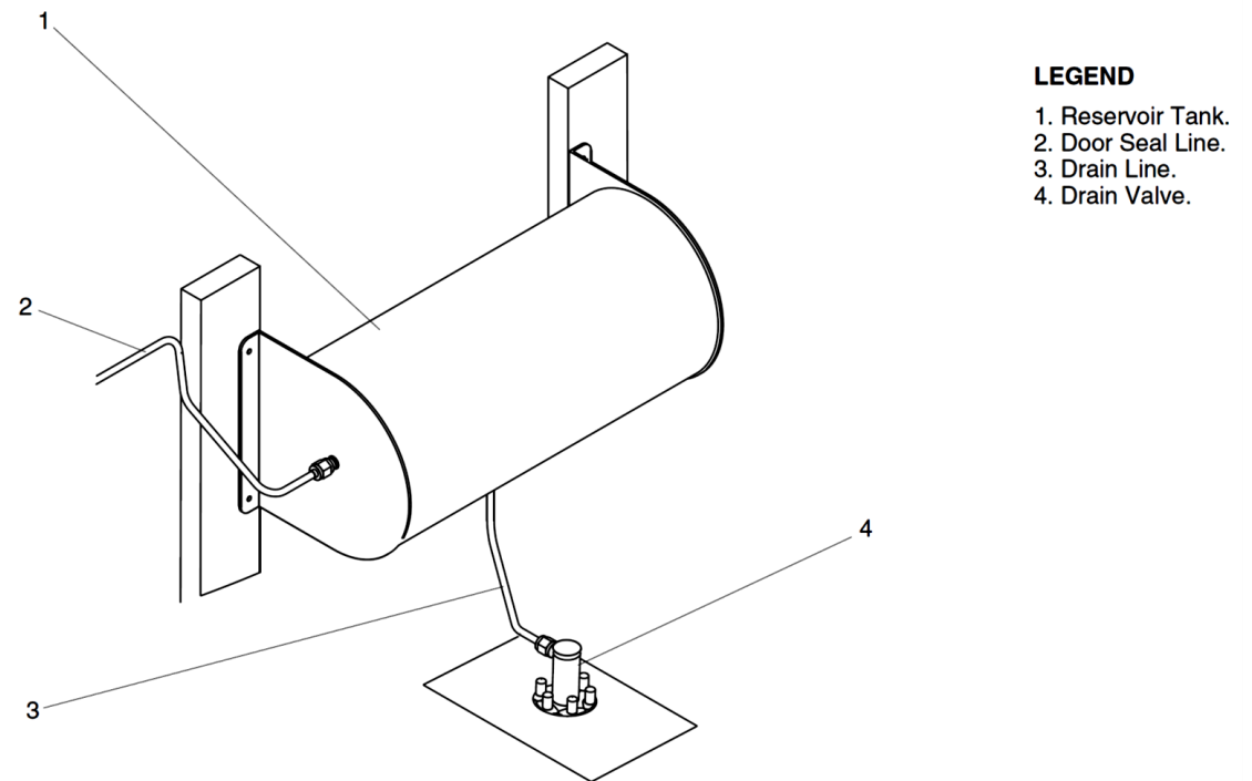
Figure 52-35 Drain Valve - Location
