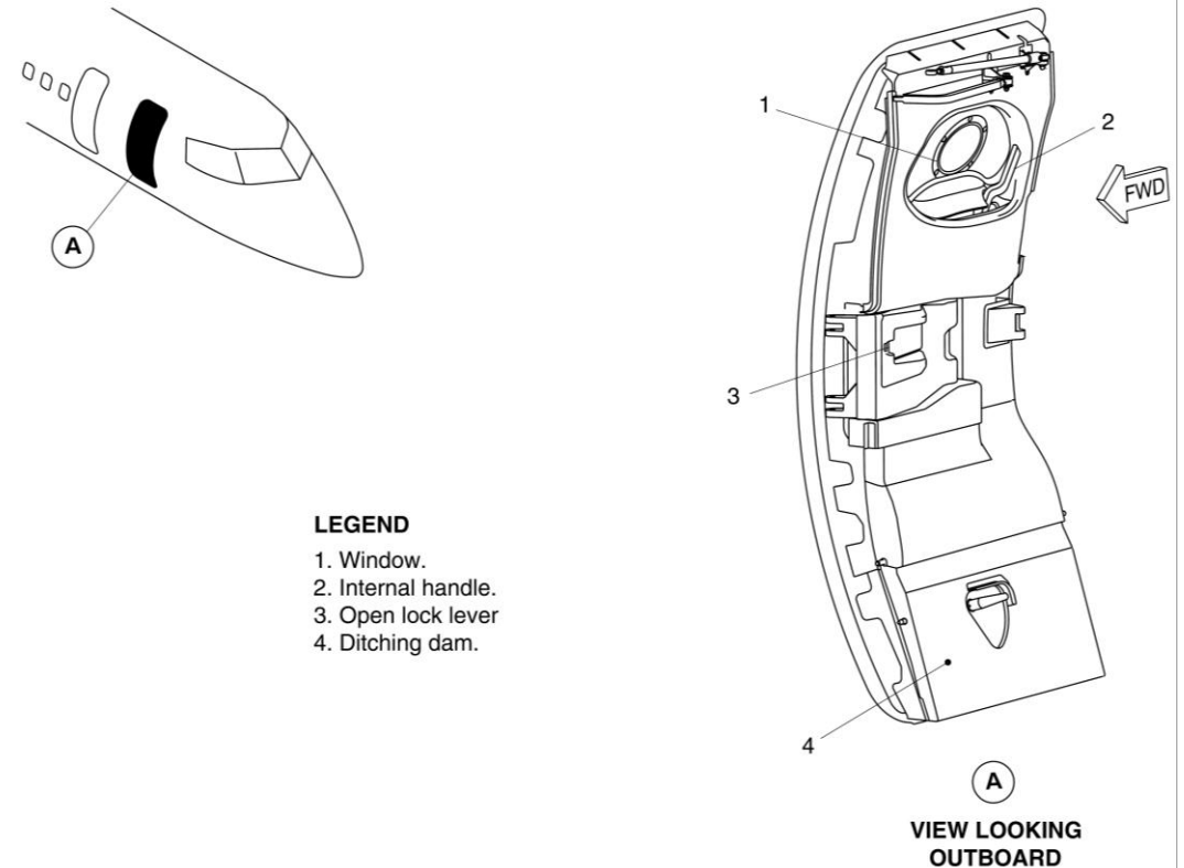
Figure 52-59 Forward Type I Emergency Exit Door – Internal View
