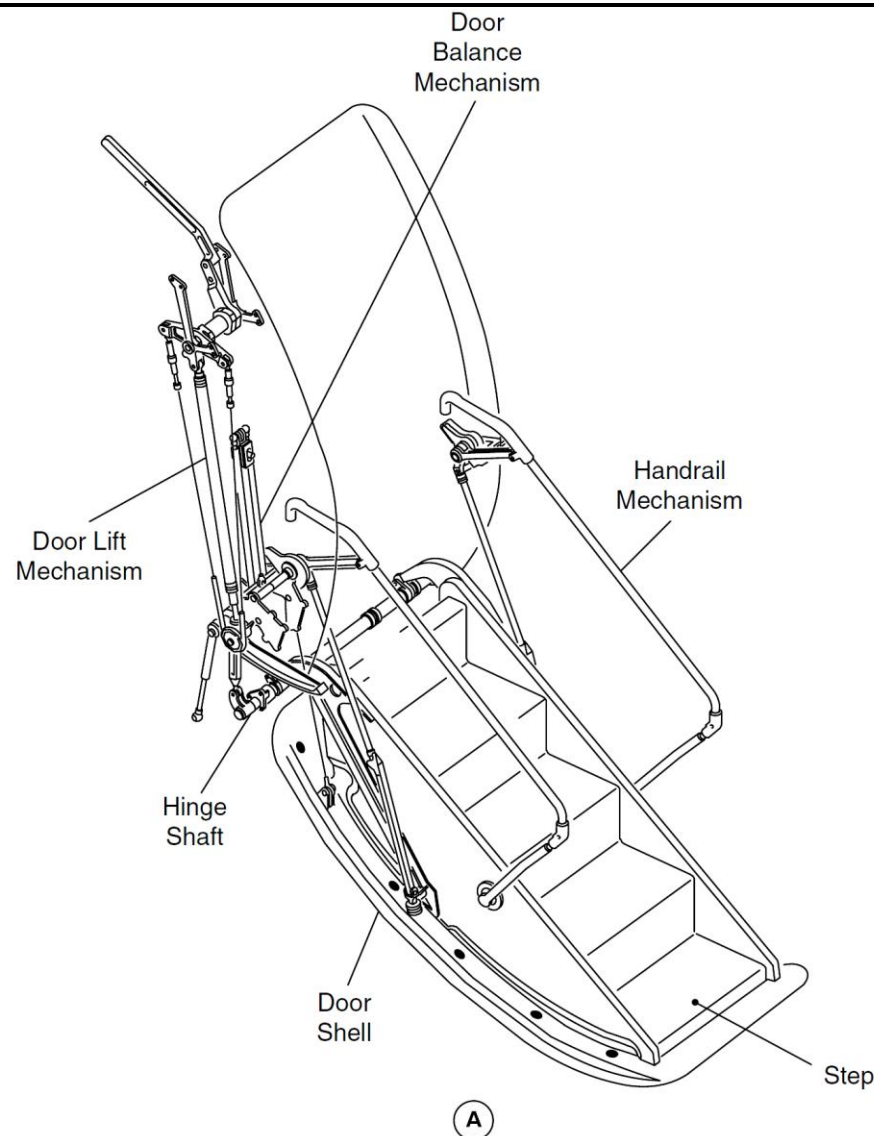
Figure 52-47 Forward Passenger Door
