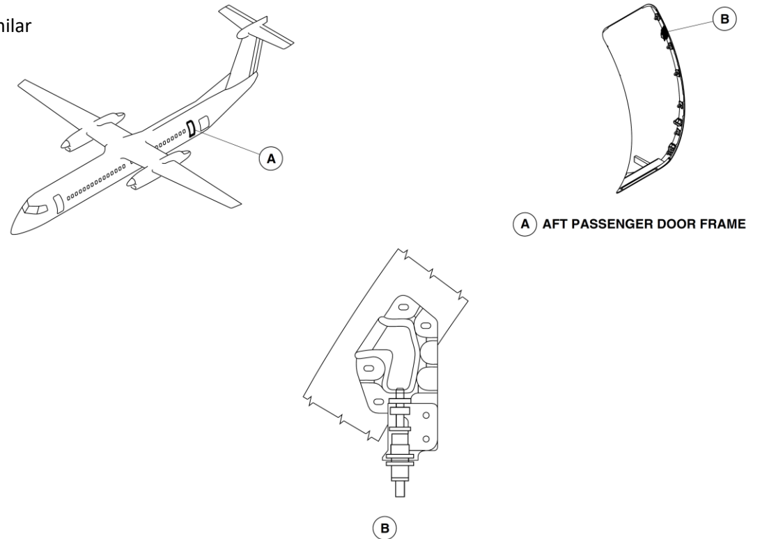
Figure 52-111 Aft Passenger Door – Closed Sensor
