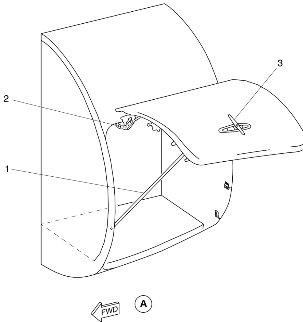
Figure 52-66 Aft Baggage Door – Open Position
