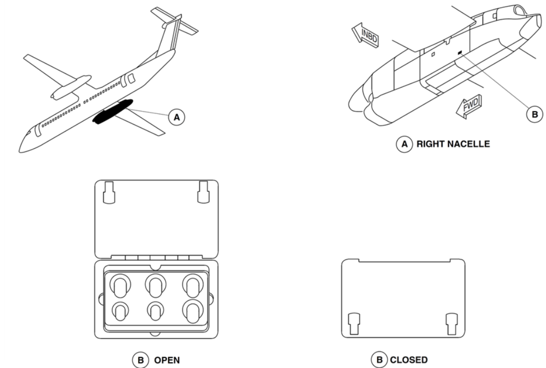
Figure 52-97 AC Electrical Ground Power Door – Detailed
