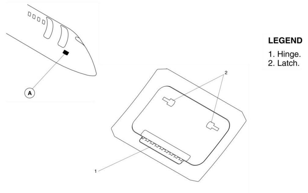
Figure 52-100 Lavatory Service Door
