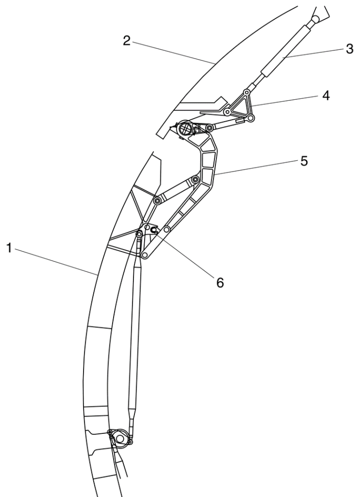
Figure 52-68 Aft Baggage Door – Lowered Position
