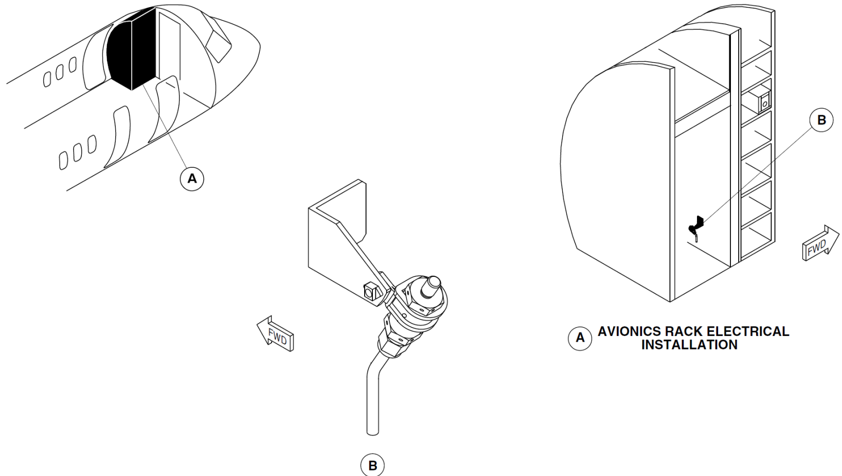
Figure 52-37 Charging Valve - Location
