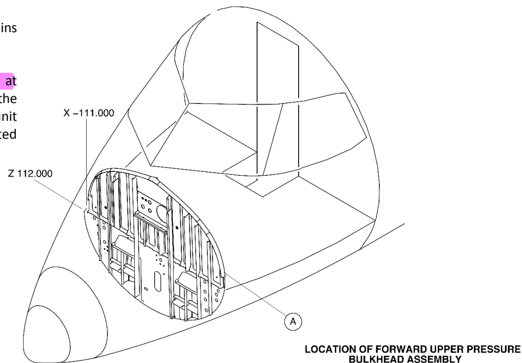
Figure 53-4 Nose Fuselage – Pressure Bulkhead
