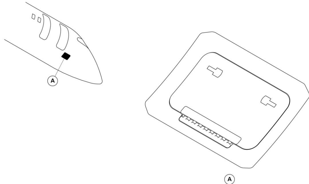
Figure 53-13 Forward Center Fuselage – Access Panels
