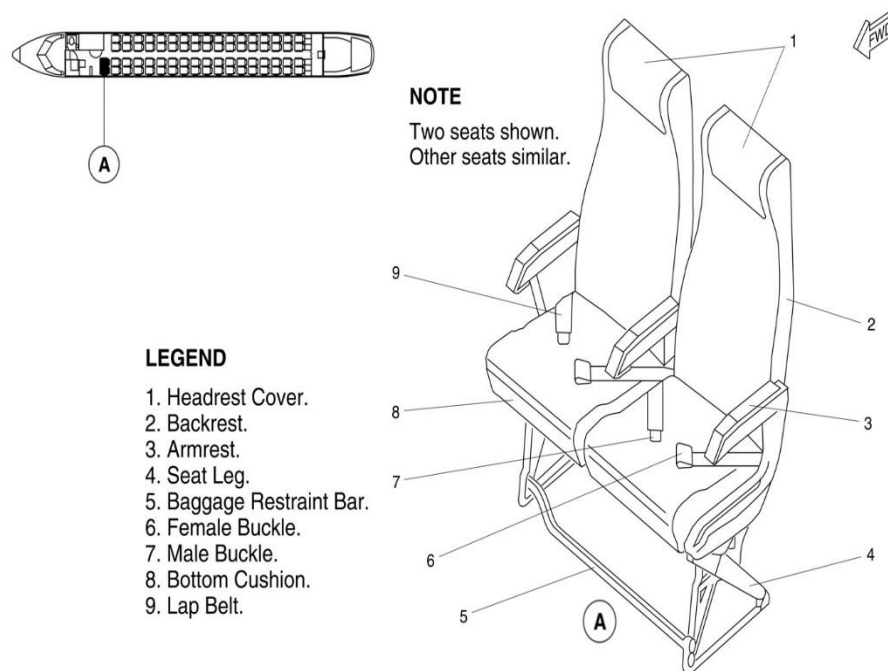
Figure 25-6 Passenger Seat
