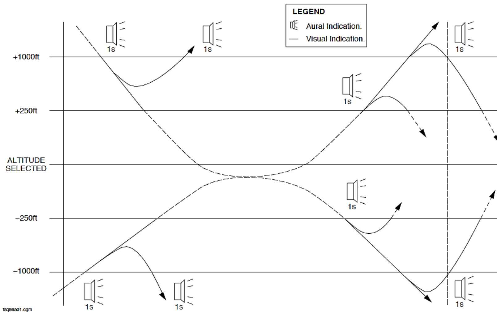
Figure - FDPS ALTITUDE ALERT
