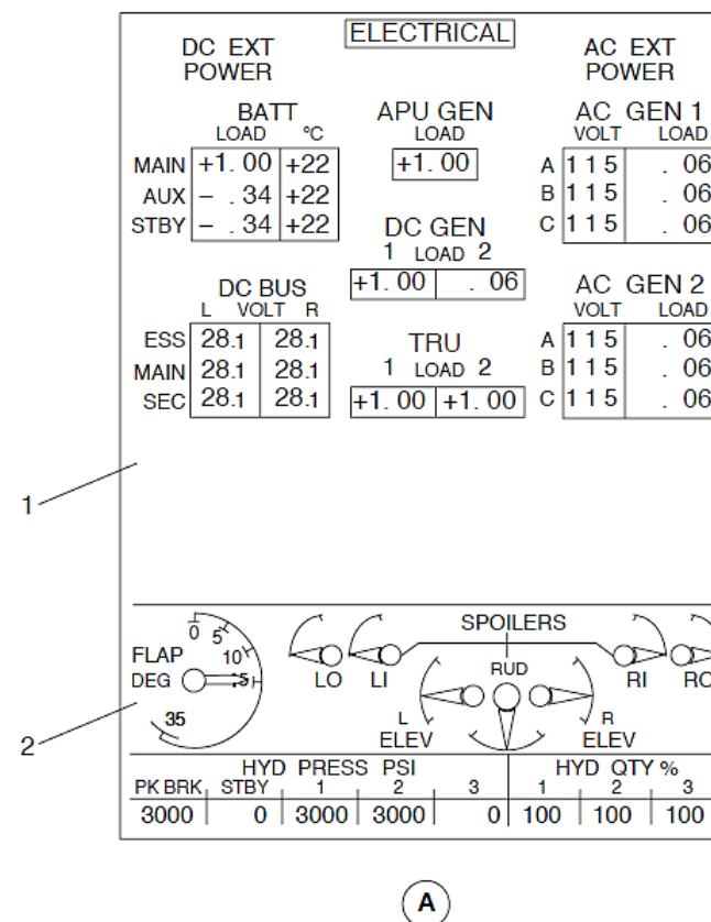
Figure - ELECTRONIC INSTRUMENT SYSTEM PERMANENT SYSTEM DATA AREA, COMPOSITE VIEW
