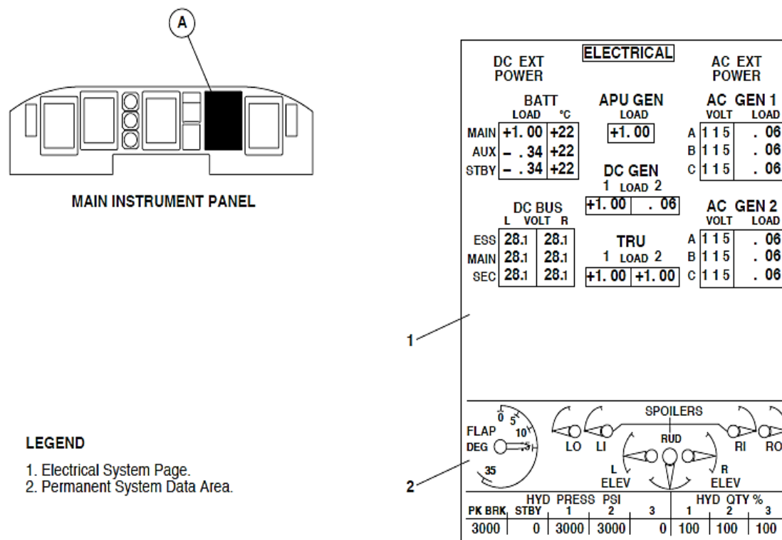
Figure - ELECTRONIC INSTRUMENT SYSTEM MFD2 INDICATIONS
