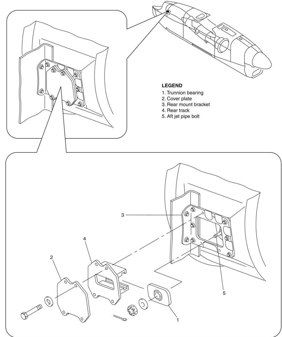
Figure 78-7 Trunnion Bearings
