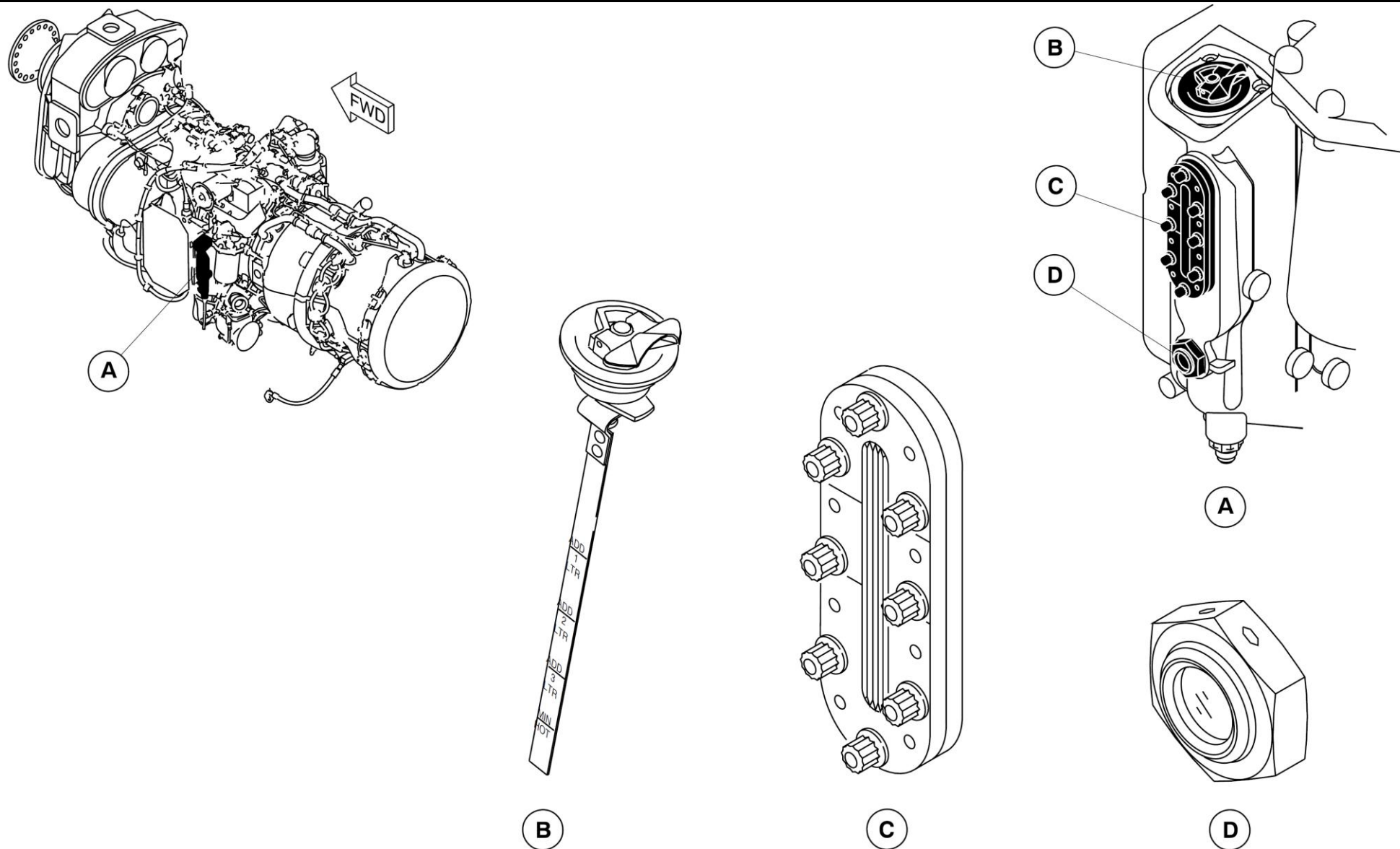
Figure 79-19 Oil Quantity Indication
