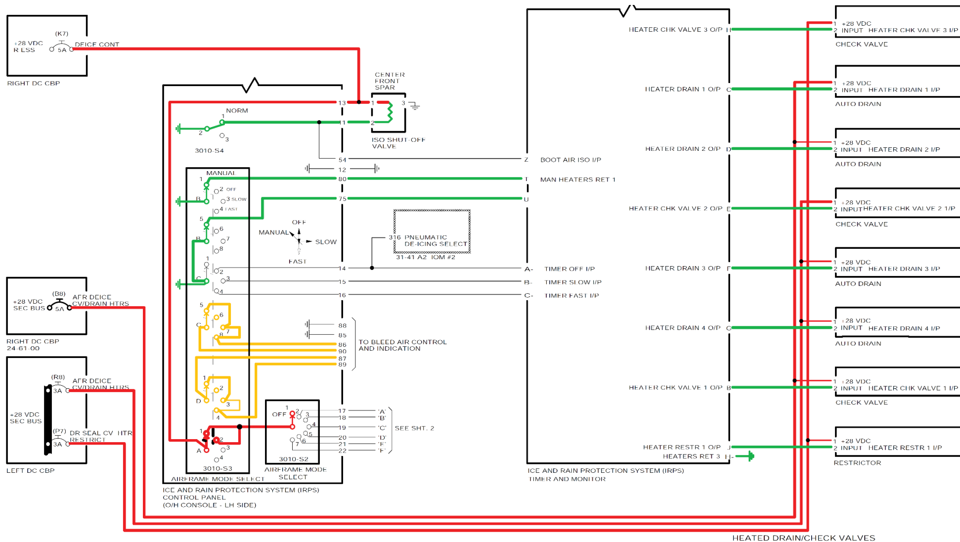
Figure 30-28 Pneumatic De-ice Electrical Schematic – Normal Operation
