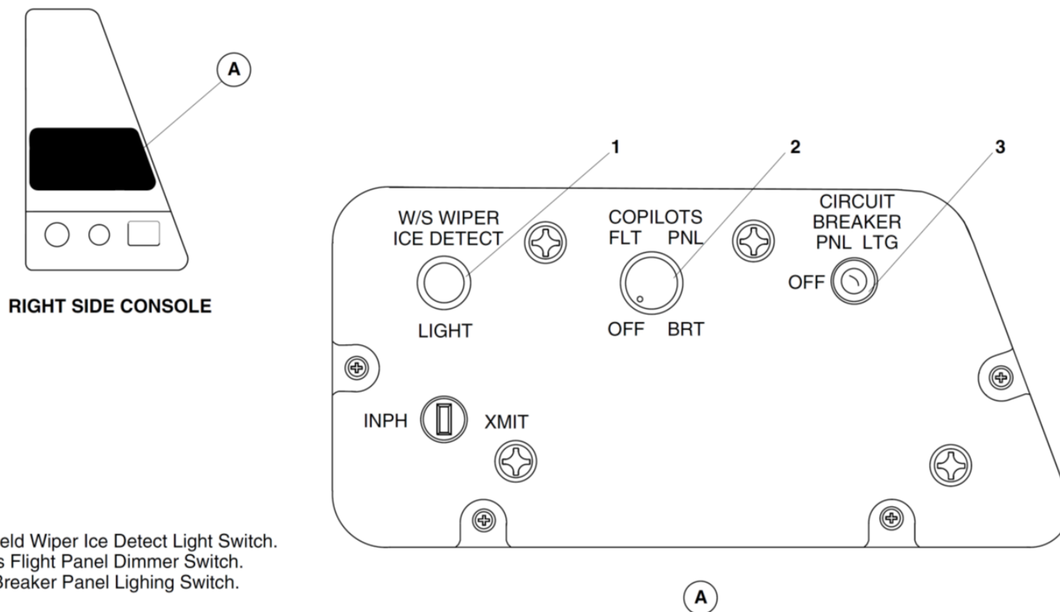
Figure 30-61 Co-Pilot Side console Panel – Location
