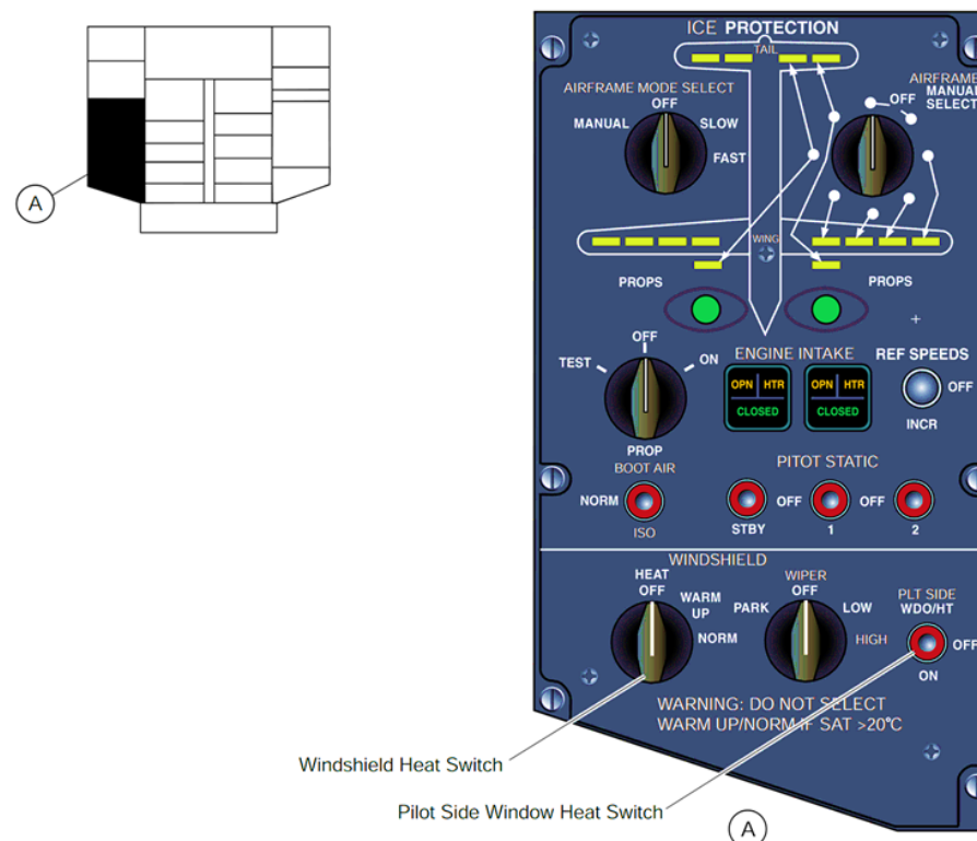
Figure 30-50 Windshield Control Panel – Location
