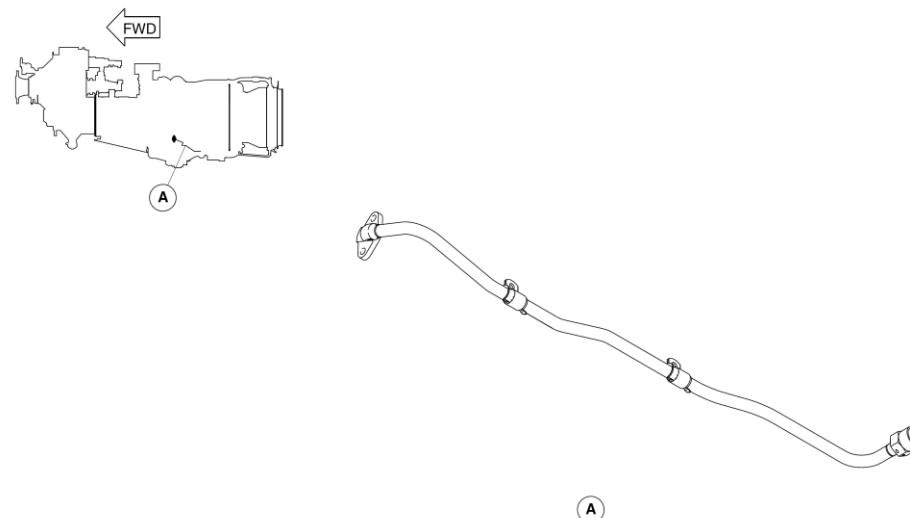
Figure 75-13 P3 Air Separator to P2.2 Bleed Valve Air Tube
